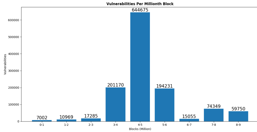
Fig. 4. Exploits Per Millionth Block
