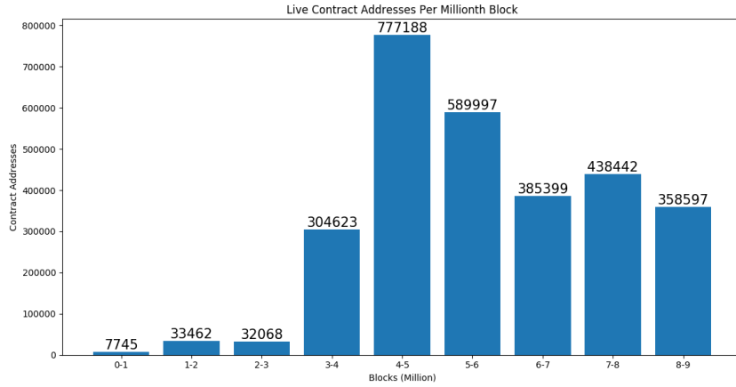
Fig. 2. Live Contract Addresses in 9 Million Blocks
