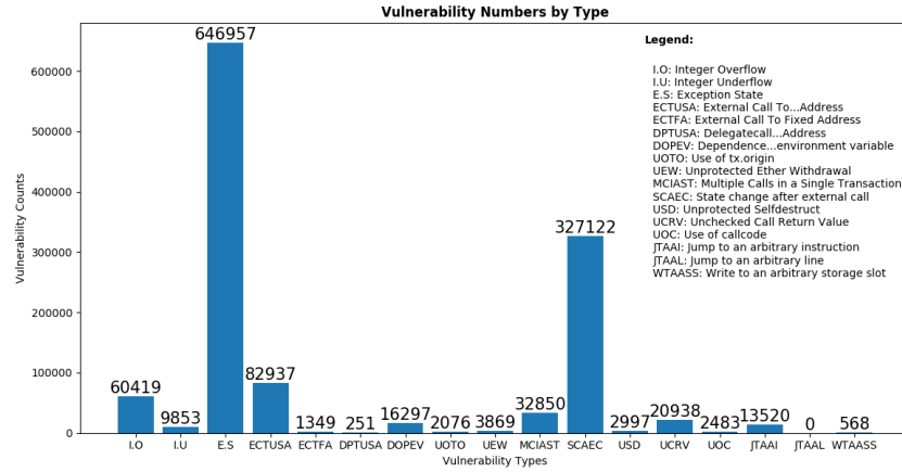
Fig. 3. Number of Vulnerabilities by Type
