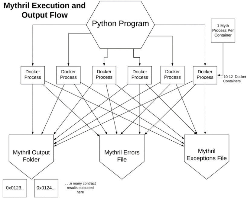
Fig. 1. High-Level Overview of Data Collection Program [9]
