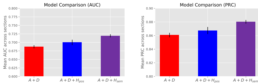
Fig. 8: Comparison of three predictive models with latent ability and difficulty parameters, and optionally using positional or semantic highlighting features, H_{pos} and H_{sem} , respectively. Error bars reflect \pm 1 SEM, corrected to remove variance due to the random factor [7]
