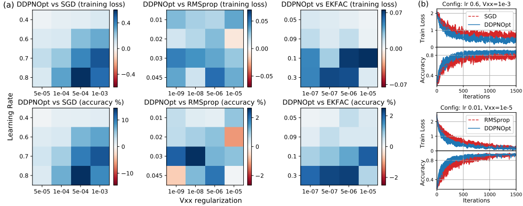
Figure 4: (a) Performance difference between DDPNOpt and baselines on DIGITS across hyperparameter grid. Blue ( resp. red) indicates an improvement ( resp. degradation) over baselines. We observe similar behaviors on other datasets. (b) Examples of the actual training dynamics.
