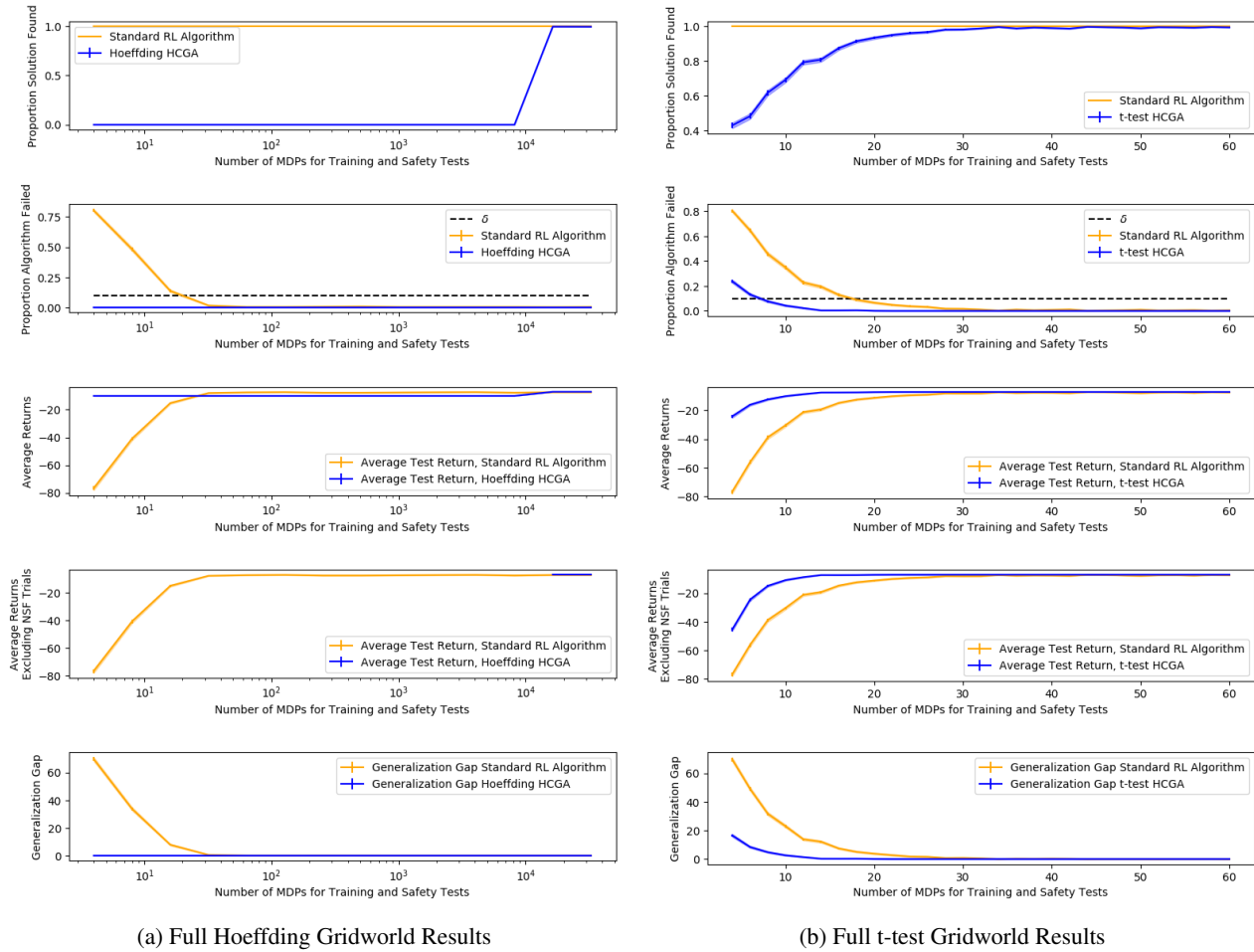
Figure 8. Full Hoeffding and t-test Gridworld Results
