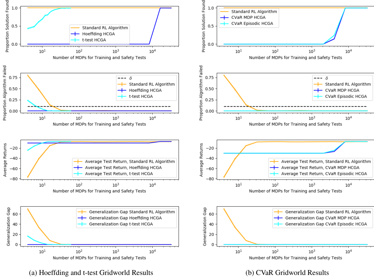
Figure 1. Generalization gridworld results. In all plots, the horizontal axis is the number of MDPs accessible for training and safety tests (that is, |M_{\text{acc}}| ). All error bars represent standard error. In all plots, the phrase “Standard RL Algorithm” represents an algorithm which does not run a safety test, and instead naively maximizes the objective. The first (top) plots show the proportion of trials in which a solution is found (that is, trials in which the algorithm did not return NSF). The second plots in these figures show the proportion of trials in which the algorithm fails; that is, the proportion of trials in which an unsafe solution is returned. In all experiments, \delta = 0.1 . The third plots in each figure show the average returns. The fourth plots show the generalization gap. These plots were generated using 1000 trials per data point (that is, 1000 trials for each location on the horizontal axis). All other details are discussed in supplementary material Section K.1.
