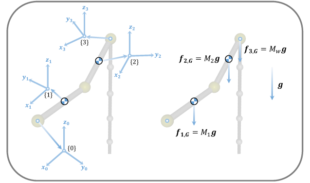
Fig. 2: Frames and the imposed gravitational forces of the simulation model. Frame 0, 1, 2 and 3 are attached to the shoulder, center of mass of the upper arm, center of mass of the forearm, and the end-effector of the upper limb model, respectively.
