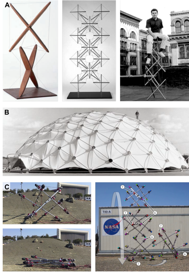
Figure 1. Tensegrity concepts were originally applied to create (A) artwork 3 and (B) lightweight architectural structures. 4 (C) Recently, roboticists have built tensegrity robots that can withstand significant impacts, such as falling from the roof of a building. 15
