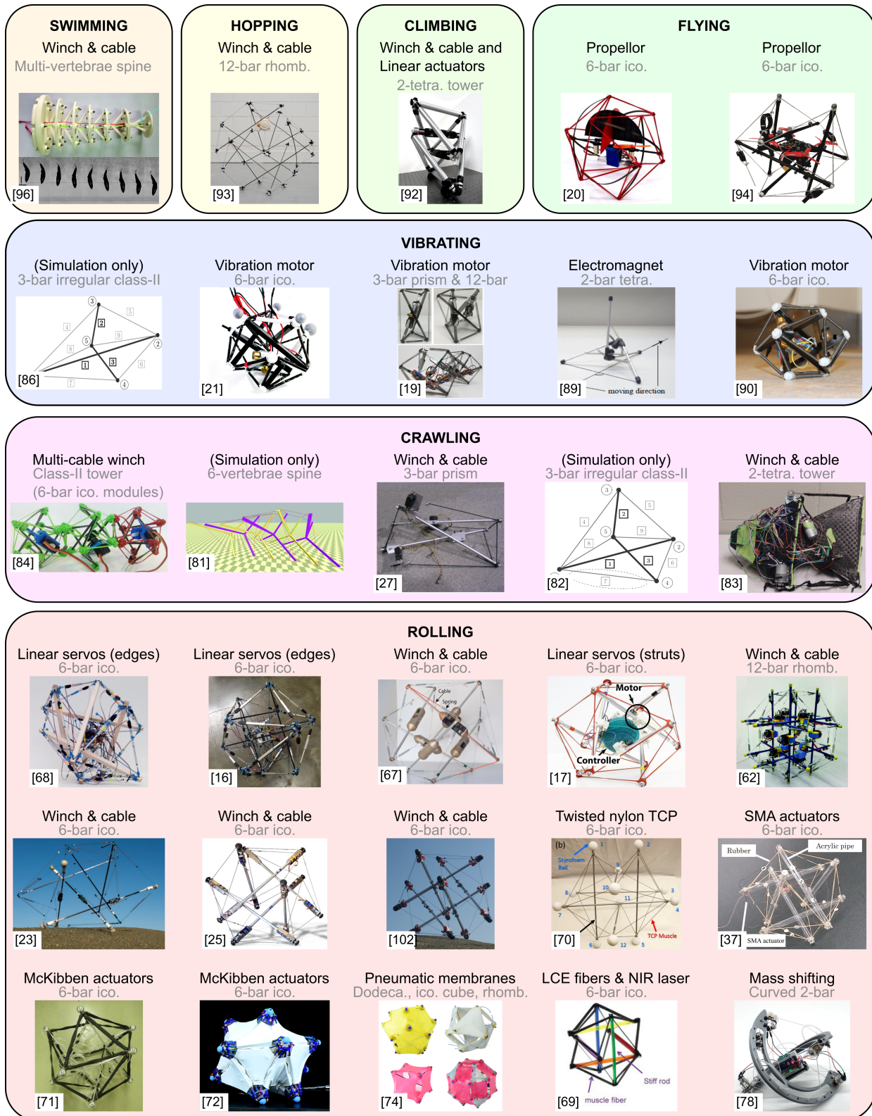
Figure 4. Representative examples of locomotion strategies utilized by tensegrity robots. Since actuation and topology are often tightly coupled with the locomotion strategy, these are also indicated for each example.
