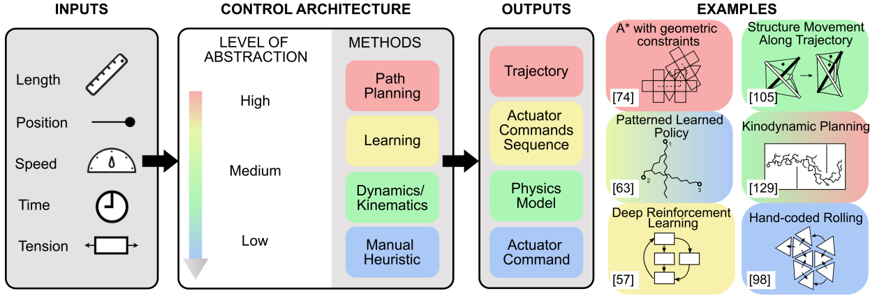
Figure 6. Tensegrity robots can be controlled at various levels of abstraction, ranging from low-level motion primitives generated from manual experimentation or physical models, to high-level motion planning to move the robot through a series of waypoints.
