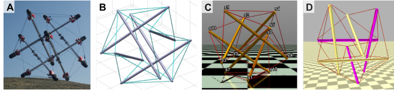
Figure 3. From left to right: SUPERball v2 15 and its model in TensegrityMATLABObjects, 44 MuJoCo 53 and NTRT. 24 TensegrityMATLABObjects can simulate dynamic motions, while MuJoCo can additionally detect rod-rod collisions, and NTRT can even detect collisions between cables and other components.
