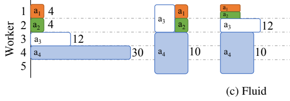
Figure 5. Toy example: default, optimal and Fluid for 4 training trials scheduled on 5 workers
