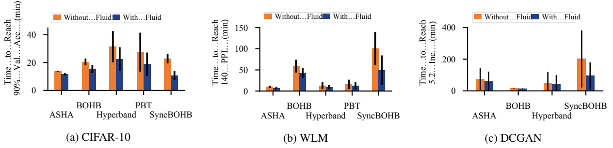
Figure 7. Time to reach target. Data averaged over 5 runs. Errorbar represents standard deviation. PBT on DCGAN did not finish in reasonable time and thus excluded from the report.
