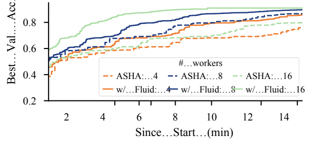
Figure 10. Validation accuracy over time for ASHA w/ and w/o Fluid on the CIFAR-10 task. Data averaged over 5 runs. Fluid is set to have 8 concurrent trials regardless of # workers.
