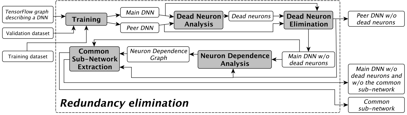
Figure 4. The redundancy elimination phase of CODE.
