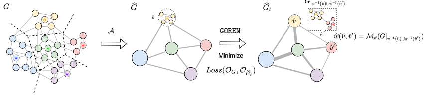
Figure 1: An illustration of learnable coarsening framework. Existing coarsening algorithm determines the topology of coarse graph \hat{G} , while GOREN resets the edge weights of the coarse graph.
