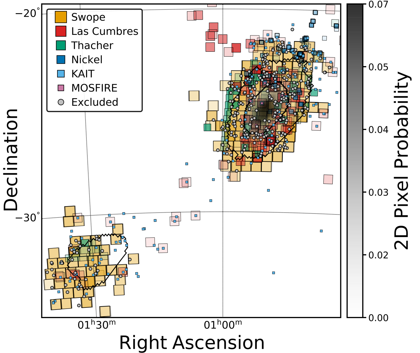
Figure 1. The LVC localization region of GW190814 with our follow-up observations from KAIT (light blue), Las Cumbres (red), Nickel (dark blue), Swope (orange), and Thacher (green) overplotted. We also show candidate counterparts imaged near the GW190814 localization region and excluded candidates (gray).
