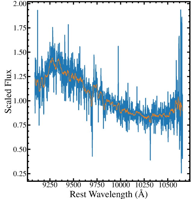
Figure 3. Keck/MOSFIRE spectrum of the GW190814 candidate counterpart AT 2019nra ( z = 0.269 \pm 0.029 ) obtained on 18 Aug. 2019 as reported by Dimitriadis et al. (2019). The spectrum is largely featureless apart from a single intermediate-width feature at a rest wavelength of 9300 Å, although this wavelength does not correspond to any known features.
