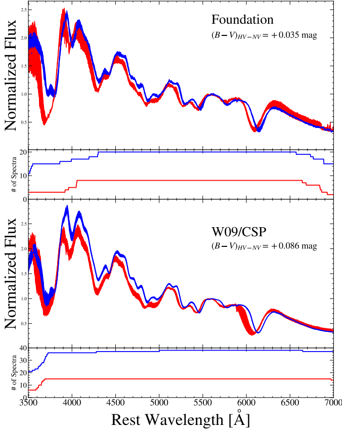
Figure 5. Composite spectra made using kaepora (Siebert et al. 2019) of Foundation and W09/CSP objects. Red lines are for high-velocity SNe and blue for normal velocity. The shaded regions are derived from bootstrap resampling of the constituent spectra as described by Siebert et al. (2019). The spectra were normalized to their median continuum between 5500–5700 Å. The number of spectra that contribute at each wavelength is shown in the bottom panels. In the upper right-hand corner, the difference in the B-V color between the high-velocity and normal-velocity subsets. Like for the color offset, the Foundation sample shows a smaller color difference in the composite spectra.
