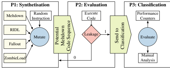
Figure 2: Transsynther phases: After mutating a new code sequence for a meltdown-style attack, the code is evaluated. If there is a leakage detected, the sample is analyzed further during the classification phase.
