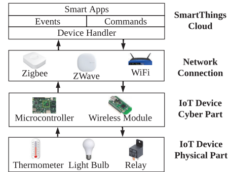
Figure 2: The SmartThings architecture.
