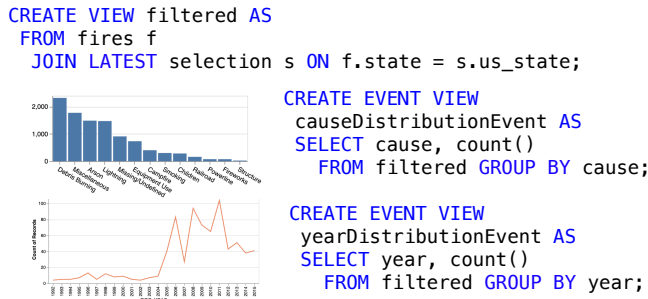
Fig. 5: An example of reuse: the filtering logic based on the selection in Fig. 2, filtered, is shared by two visualizations. DIEL analyzes the query plan and materializes filtered to avoid evaluating it twice.
