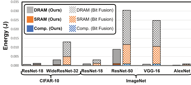
Figure 9: Energy breakdown of our 2-in-1 Accelerator and Bit Fusion on six networks executed with 4-bit X 4-bit.
