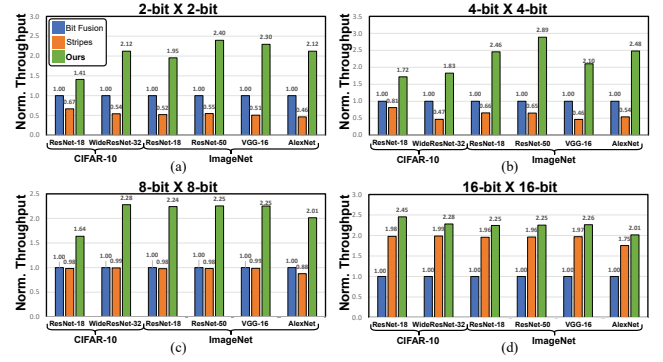
Figure 7: Normalized throughput comparison among Bit Fusion, Stripes, and our 2-in-1 Accelerator on top of six networks and four execution precisions.
