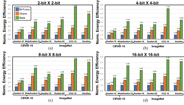
Figure 8: Normalized energy efficiency comparison among Bit Fusion, Stripes, and our 2-in-1 Accelerator on top of six networks and four execution precisions.
