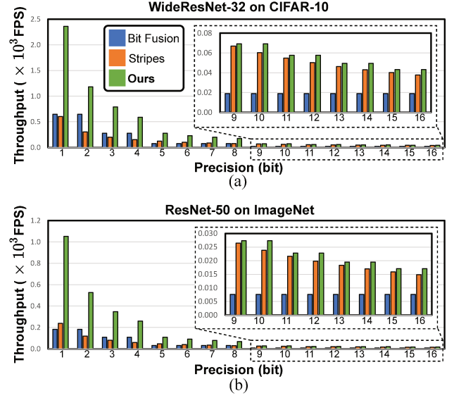
Figure 10: Throughput under different precisions of Bit Fusion, Stripes, and our 2-in-1 Accelerator for accelerating WideResNet-32 on CIFAR-10 and ResNet-50 on ImageNet.
