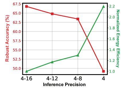
Figure 11: 2-in-1 Accelerator 's instant robustness-efficiency trade-off on top of WideResNet-32 and CIFAR-10.
