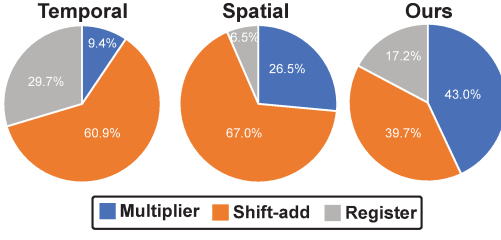
Figure 3: Area breakdown of the MAC units based on SOTA temporal/spatial designs and our proposed design.
