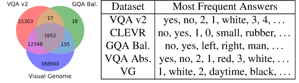
Figure 3. Venn diagram of answer vocabulary of three datasets. A large portion of answers are not shared across datasets, and the distribution ( e.g. most frequent answers) may differ as well.
