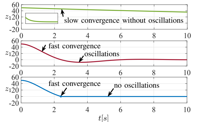
Fig. 1. Comparison of the performance of the heavy ball method, with large value of \lambda , Nesterov's accelerated gradient descent, and the proposed logic-based algorithm. The objective function is L(z_1) = z_1^2 . Top: the heavy ball algorithm, with large \lambda , converges very slowly. Top inset: zoomed out view of heavy ball. Middle: Nesterov's accelerated gradient descent converges quickly, but with oscillations. Bottom: our proposed logic-based algorithm yields fast convergence, with no oscillations.
