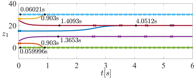
Fig. 2. The evolution of z_1 over time for the hybrid system \mathcal{H} , for the objective function L(z_1) = \frac{z_1^2(z_1-10)^2(z_1-20)^2(z_1-30)^2}{10,000} , with \mathcal{A}_{1\min} = \{0, 10, 20, 30\} , \mathcal{A}_{1\max} = \{5(3 - \sqrt{5}), 15, 5(3 + \sqrt{5})\} , and \varepsilon_1 = 0.05 , \varepsilon_2 = 0.06 , \rho_1 = 0.05 , \rho_2 = 0.06 , \nu = 1 , \lambda = 145 , and \gamma = \frac{3}{4} . This plot shows different solutions, starting from different initial conditions. Solutions start at local maxima at z_1(0,0) = 15 , z_1(0,0) = 5(3 - \sqrt{5}) , and z_1(0,0) = 5(3 + \sqrt{5}) , as well as at the points z_1(0,0) = 6 , z_1(0,0) = 24.5 , z_1(0,0) = -1 , and z_1(0,0) = 31 , which are neither maxima nor minima. All solutions start with z_2(0,0) = 0 and q(0,0) = 0 . Times when each solution converges to within 0.01 of \mathcal{A}_{1\min} are marked with black dots and labeled in seconds. Jumps are labeled with asterisks.
