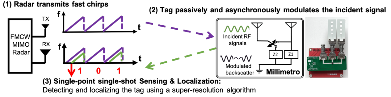
Figure 4: System Overview
