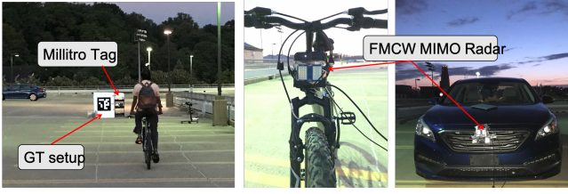
Figure 15: Millimetro was tested in 3 mobile environments: walking, biking and driving.
