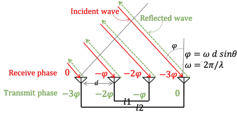
Figure 3: The Van Atta retro-directive array is a passive design that reflects back any incident wave in reverse, parallel to the direction of incidence.
