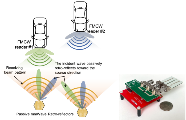
Figure 1: Millimetro is an ultra-low-power mmWave retro-reflector that supports accurate localization at long-range. Millimetro gets its long-range from reflecting back incident waves directionally towards the reader, and accuracy from the large bandwidth available at mmWave.
