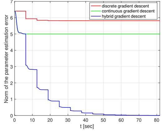
Fig. 1. Evolution of the norm of the parameter error using continuous, discrete and hybrid gradient algorithms.
