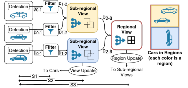
Figure 3: An exemplar of situation awareness applications – Connected Vehicles. Cars in the same spatial locale have their individual views fused by the sub-regional view; Regional view fuses sub-regional views of adjacent spatial locales.
