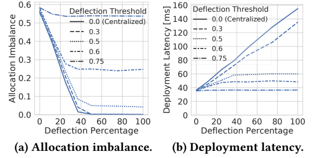
Figure 8: Trade-off in S-App request handling at proximal \mu DC vs. at central controller.
