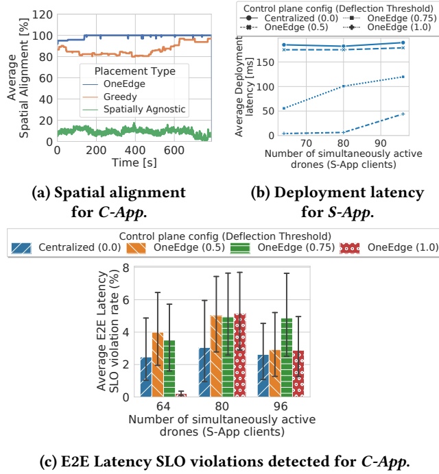
Figure 9: Evaluation of E2E situation awareness applications.
