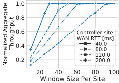
Figure 5: Impact of Pipelining on Aggregate Throughput.
