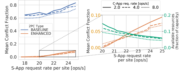
Figure 6: MCF of baseline and enhanced 2PC for typical S-App and C-App request rates from the SF cabs dataset (Table 2). The blow-up shows the increase in MCF and the \mu DC’s remaining available resources for enhanced 2PC.
