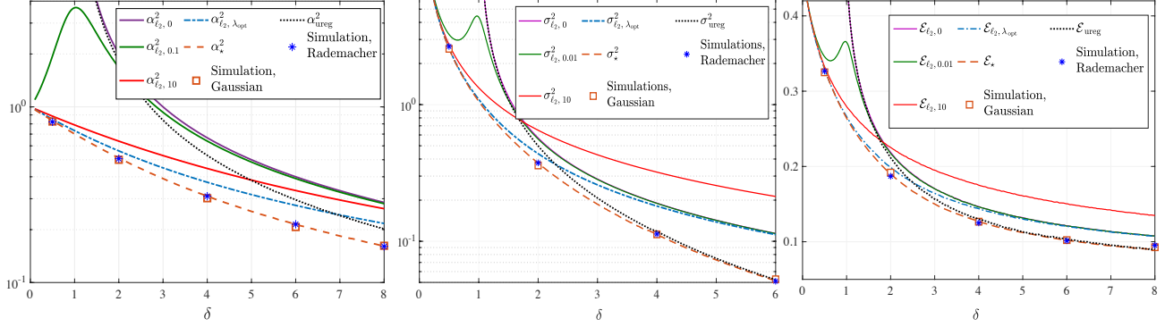
Figure 1: The lower bounds on error derived in this paper, compared to RLS for the linear model with Z \sim \text{Laplace}(0, 1) (Left), and for the binary Signed model(Middle) and binary Logistic model with \|\mathbf{x}_0\| = 10 (Right). The markers denote the empirical performance of the optimally tuned RERM as derived in Lemmas 2.1 and 3.1 for Gaussian and Rademacher data. See Section G for additional numerical results.
