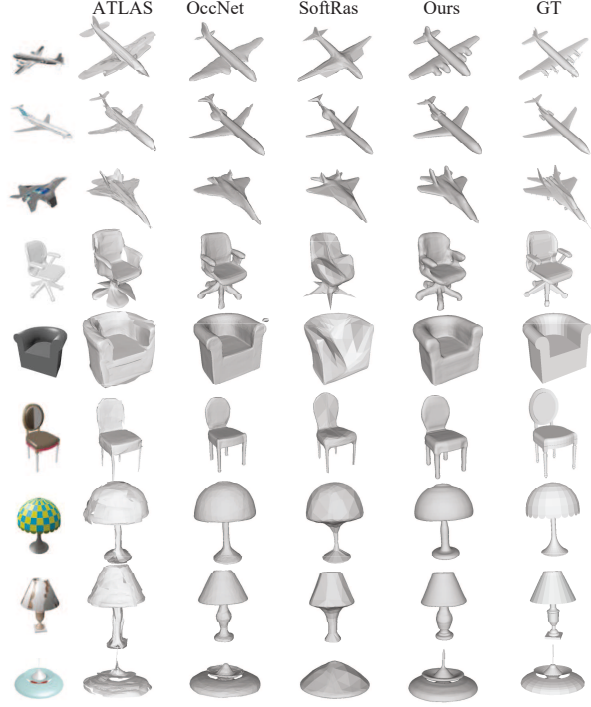
Figure 7. Comparison in single image reconstruction.
