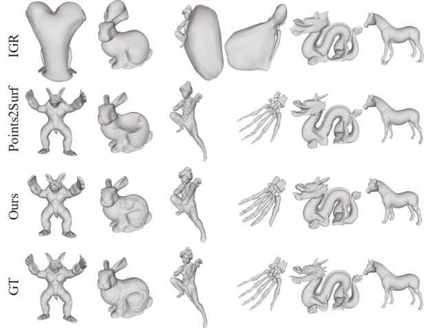
Figure 4. Comparison under FAMOUS in surface reconstruction.
