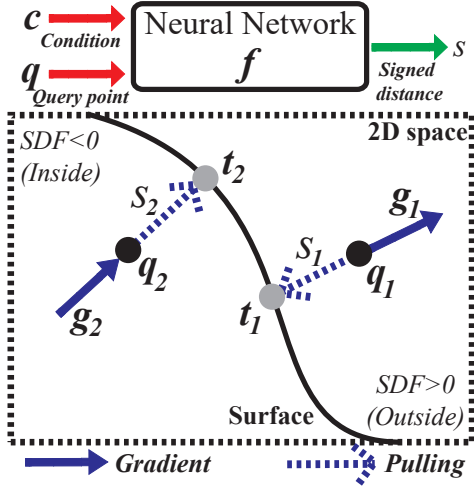
Figure 1. Demonstration of pulling surrounding 2D space to a surface, where gradients \mathbf{g}_i and signed distance value s are from neural network \mathbf{f} .
