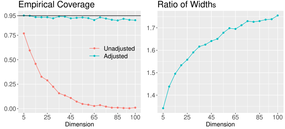
Figure 2: Comparison of unadjusted and simultaneous inference when selecting one covariate out of d . The comparison is based on 1000 replications for each dimension d . The right panel shows the ratio of the width of simultaneous confidence interval 16. to that of the unadjusted confidence interval 17., i.e., \hat{K}_\alpha/z_{\alpha/2} .
