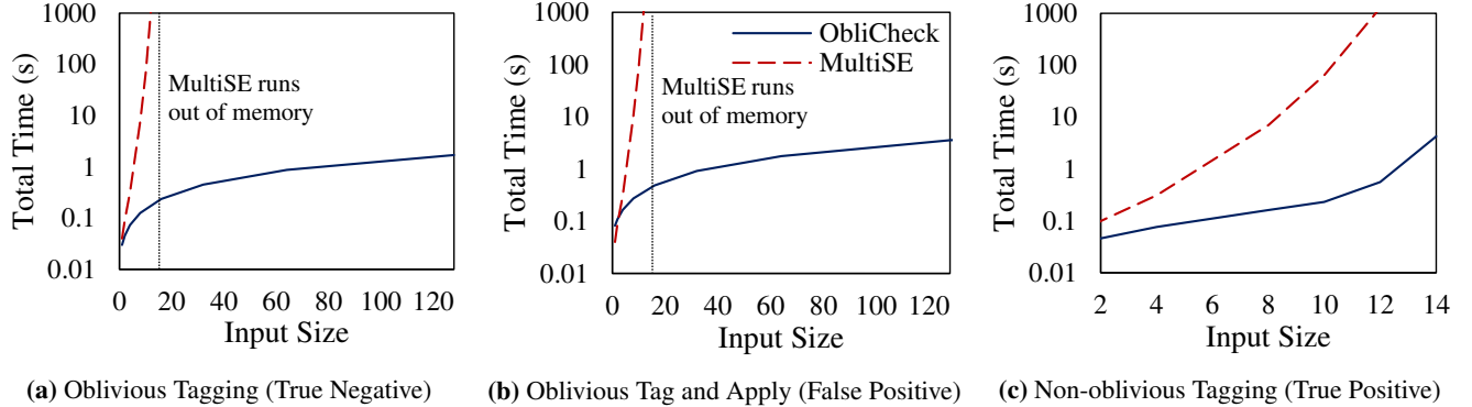
Figure 6: Total analysis time of MultiSE (conventional state merging) and ObliCheck (domain-specific merging followed by iterative state unmerging) over Tag, Tag&Apply, and Tag (Non-oblivious). The total time of MultiSE grows exponentially until the input size 16 and fails to finish due to out of memory error after then when it analyzes Tag and Tag&Apply. The total analysis time of ObliCheck grows linearly without out of memory error. The total time of ObliCheck blows up exponentially when it checks the non-oblivious Tag algorithm. This is because state merging is not possible after unmerging merged state and the size of state exponentially grows as MultiSE does.
