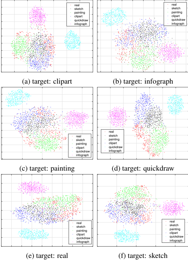
Figure 4: The t-SNE visualization of dynamic coefficients \Pi = \{\pi_i^l(x)\} when DRT is trained with target domain- ‘clipart’, ‘infograph’, ‘painting’, ‘quickdraw’, ‘real’ and ‘sketch’. (Best view in color)
