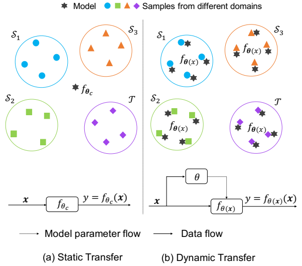
Figure 1: Static Transfer vs. Dynamic Transfer. (a) ‘Static Transfer’ implements domain adaptation with a static model f_{\theta_c} , which has fixed parameters \theta_c to average domain conflict. (b) ‘Dynamic Transfer’ ( f_{\theta(x)} ) adapts the model parameters \theta(x) according to samples, which generates a different model per sample and turns multi-source domain adaptation into single-source domain adaptation.
