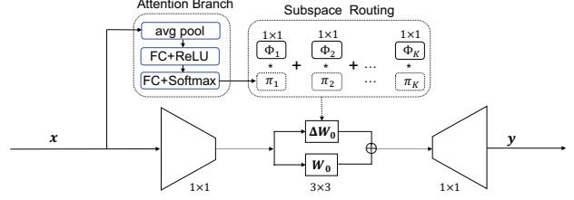
Figure 3: Subspace routing of DRT: dynamic coefficients are generated by a dynamic branch given the input x . Each dynamic coefficient \pi_i(x) is then multiplied by a matrix \Phi_i , and the K matrices are aggregated as the residual kernel- \Delta W_0(x) . For channel attention, softmax is replaced by sigmoid and the resulting coefficients in \Lambda(x) are multiplied to corresponding channels of W_0 .
