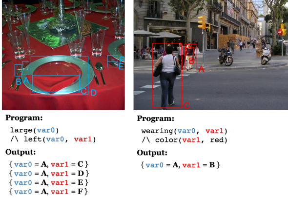
Figure 6. Examples from the GQA dataset (Hudson & Manning, 2019). We show bounding boxes for objects relevant to the query. In both cases, the target object is object A. We show the program synthesized using our approach based on the ground truth scene graphs, along with the possible variable bindings.
