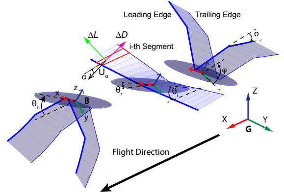
Fig. 2. Dynamic wing-body system with twist and folding capability. The wing mass is considered to be distributed along the armwing only. The folding motion ( \sigma ) is specified as a relative rotation between hand and armwing. The twist is defined as a linear distribution of increasing pitching angle from root ( \theta_r ) to tip ( \theta_i , with indices i = wing tip).
