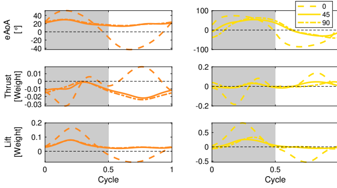
Fig. 5. Impact of fold alone on the aerodynamics at 5 m/s. The orange and gold color represent a segment in the armwing and handwing respectively. The dark shades indicate downstroke. We assumed the axis of wing fold is exactly at the half-semispan, and that the folding is an additional time-varying relative rotation (with amplitude being \Sigma ) of the handwing with respect to the armwing. Here, three cases of increasing maximum folding angles \Sigma = 0, 45 and 90 are presented.
