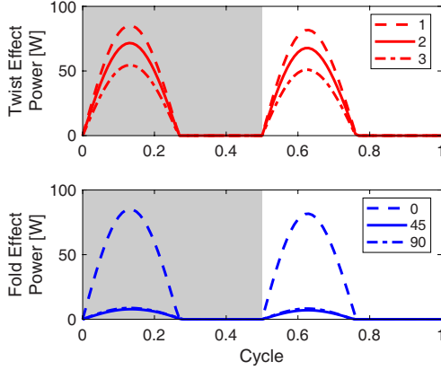
Fig. 6. Temporal energy expenditure of the flapping wing system at 5 m/s, for twist \xi = 1, 2 and 3 , or fold \Sigma = 0, 45 or 90^\circ . The dark shades indicate downstroke.
