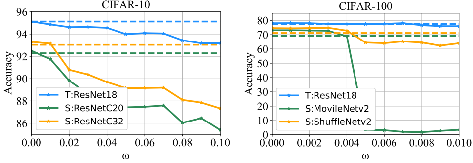
Figure 3: Ablation study w.r.t \omega on CIFAR-10 and CIFAR-100. The initials “T” and “S” in the legend represent teacher networks and student networks, respectively. The dash-line represents the accuracy that the model is normally trained.
