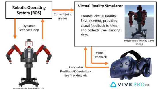
Figure 1. Schematic of communication between Baxter and VR
