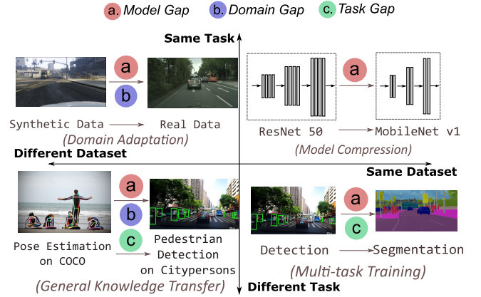
Figure 1: Illustration of different settings for transferring a well-trained teacher network to a student network, with the model, domain, and task gaps defined in this paper. We validate the generality of the proposed hybrid forward extensively on diverse knowledge transferring settings in the experiments.
