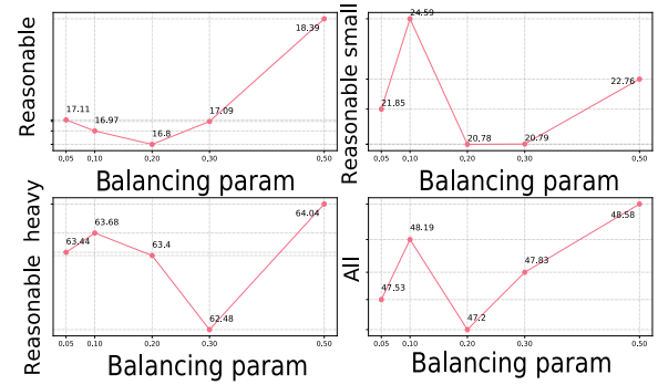
Figure 9: Results on general knowledge transfer with different fixed balancing parameters.
