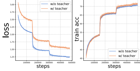
Figure 5: Training loss and training accuracy with and without the teacher network on ImageNet with ResNet-50 as the teacher and MobileNet-v1 as the student.
