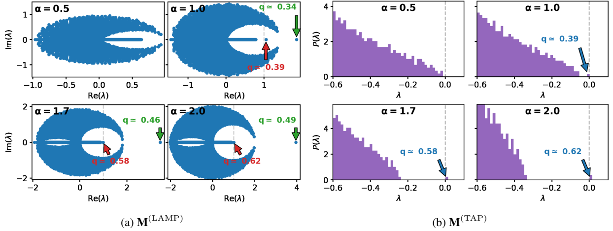
Figure 7: Transition in the spectra of \mathbf{M}^{(\text{LAMP})} and \mathbf{M}^{(\text{TAP})} for \Phi being the product of two complex Gaussian matrices, and a noiseless phase retrieval channel, for the recovery of a natural image. For \alpha > \alpha_{\text{WR,Algo}} = 0.5 , we indicate the approximate overlap q corresponding to the relevant eigenvalues.
