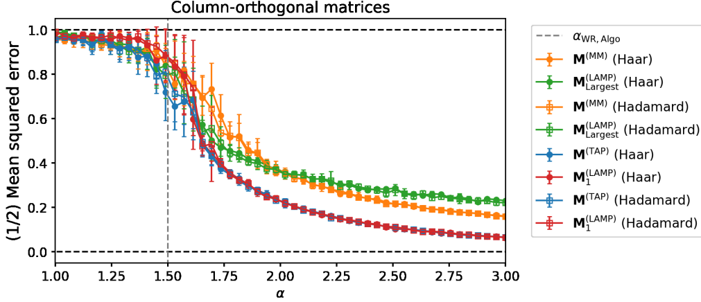
Figure 1: Mean squared error achieved by our spectral methods and a naive version of the spectral method of [MM19] for real column-orthogonal sensing matrices and a noiseless channel. We give the performance on uniformly sampled column-orthogonal matrices as well as randomly subsampled Hadamard matrices. The simulations were done using m = 8192 , and the error bars are taken over 10 instances.
