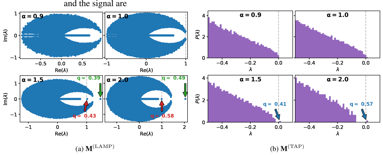
Figure 6: Transition in the spectrum of \mathbf{M}^{(\text{LAMP})} and \mathbf{M}^{(\text{TAP})} for a complex Gaussian \Phi and a noiseless phase retrieval channel. For \alpha > \alpha_{\text{WR,Algo}} = 1 , we indicate the approximate overlap q corresponding to the relevant eigenvalues.
