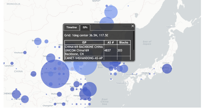
Fig. 5. An example of the pop-up's second tab which is rendered when the user selects Laiwu District, Laiwu, Shandong, China on 2020-03-11 (Section III-F).
