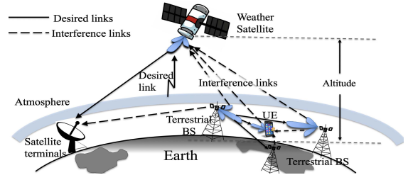
Fig. 5. Satellite and Terrestrial networks, illustrating the interference between weather satellites (passive) and terrestrial communication (active) systems.
