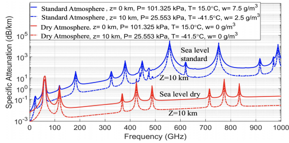
Fig. 2. Atmospheric absorption beyond Friis free space path loss [18] at z = 0 km height (sea level) and z = 10 km height (10 km above the sea level), computed from models in [16].
