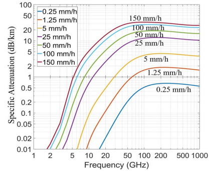
Fig. 3. Rain attenuation beyond natural FSPL in dB/km over frequency at various rainfall rates using ITU models [16], [19], [20].
