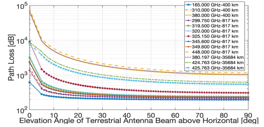
Fig. 4. Total path loss from ground terminals to satellite NGS O EESS altitudes (without antenna gains) computed from models in [16], [24].
