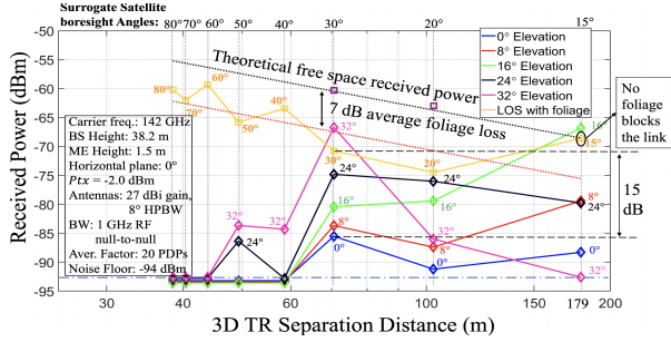
Fig. 8. The rooftop base station (38.2 m above the ground) received power vs. different distances and different elevation angles from ground users (1.5 m above the ground) at 142 GHz.
