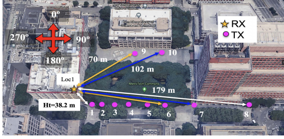
Fig. 7. Rooftop surrogate satellite measurement campaign. The surrogate satellite (and backhaul) receiver RX location is at 38.2 m above the ground on the rooftop identified as a yellow star. Ten mobile TX locations on the ground are identified as purple circles. The LOS elevation pointing angles from TX1-8 to the RX location are 80^\circ to 15^\circ , respectively.
