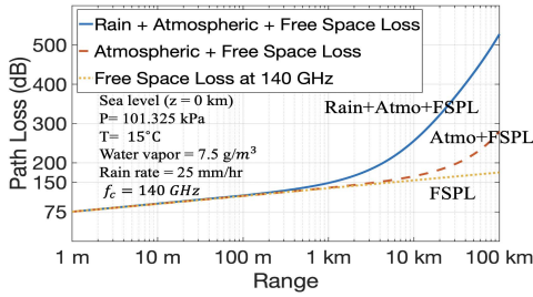
Fig. 6. Total path loss at 140 GHz ( 0^\circ elevation angle) without antenna gains including free space path loss (FSPL), rain attenuation, and atmospheric absorption on a terrestrial path using models in [16].
