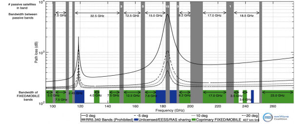
Fig. 1. Key ITU spectrum allocation above 100 GHz with RR5.340 prohibited bands, unlicensed/EESS/RAS sharing bands, and coprimary fixed/mobile bands, from millimeter wave coalition.
