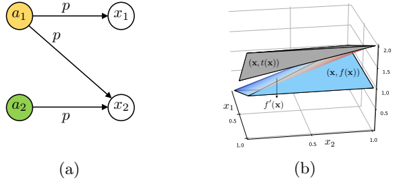
Figure 2: (a): p \in (0.5, 1) is the weight parameter. (b): Construct \mathcal{S} and \mathcal{T} when f(\mathbf{x}) = \max\{x_1, x_2\} . The gray shaded region is the set \mathcal{T} (we actually plot the convex hull of all points (\mathbf{x}, t(\mathbf{x})) ), while the light sky blue is the set \mathcal{S} . The color hyperplane is exactly f'(\mathbf{x}) = x_1 + x_2 .
