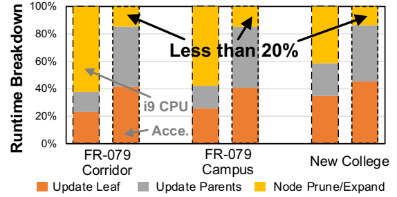
Fig. 10: Runtime breakdown in the accelerator and CPU.
