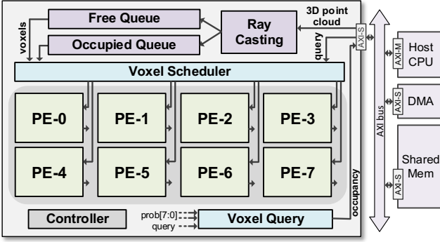
Fig. 7: Overview of the proposed OMU accelerator.
