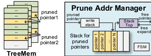
Fig. 6: Dynamic prune address manager.
