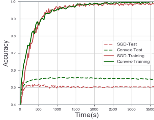
(a) CIFAR-10
