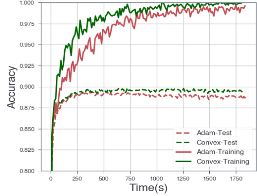
(b) Fashion-MNIST
