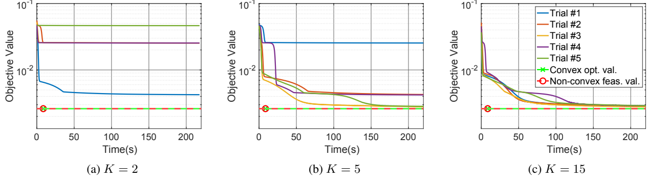
Figure 4: Training cost of a three-layer architecture trained with SGD (5 initialization trials) on a synthetic dataset with (n, d, m_1, \beta, \text{batch size}) = (5, 2, 3, 0.002, 5) , where the green line with a marker represents the objective value obtained by the proposed convex program in (12) and the red line with a marker represents the non-convex objective value in (4) of a classical ReLU network constructed from the solution of convex program as described in Proposition 1. Here, we use markers to denote the total computation time of the convex optimization solver.
