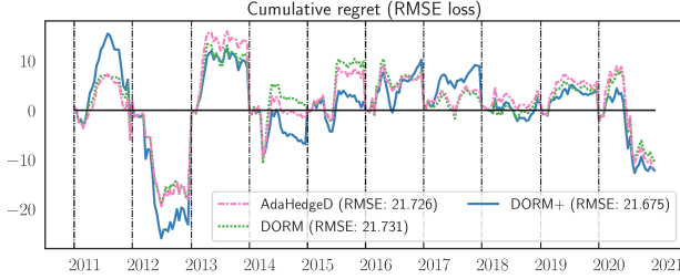
Figure 1: Overall performance: Yearly cumulative regret under RMSE loss for the Precip. 3-4w task. The zero line corresponds to the performance of the best input model in a given year.
