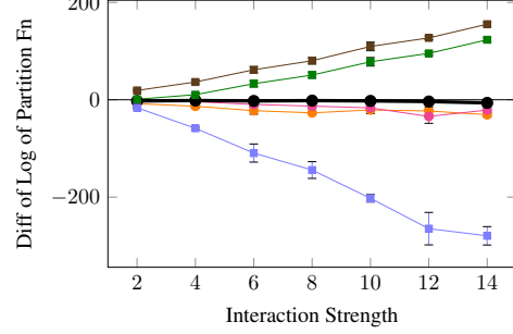
(b) 8 \times 8 Ising model with mixed interactions. We plot the difference from ground truth (line at 0).
