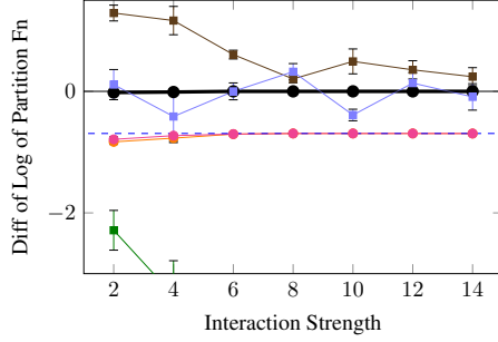
(a) 4 \times 4 Ising model with positive interactions. We plot the difference from ground truth (black line at 0). MF-VI approaches \ln(1/2) (dotted line) since it only covers one of two symmetric modes for the positive interaction case.
