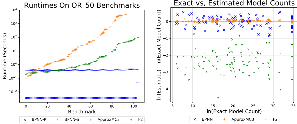
Figure 4: Left: cactus plot of runtimes for the 105 instances in the ‘or_50’ category solved by BPNN, F2, and ApproxMC3. BPNN-P denotes the time taken to run BPNN in parallel on a GPU divided by the number of instances per batch (batch size=103). Median speedups of BPNN-P over F2 and ApproxMC3 among the plotted benchmarks are 248 and 3,689 respectively. BPNN-S denotes the time taken to run BPNN sequentially on each instance (using a CPU). Median speedups of BPNN-S over F2 and ApproxMC3 among the plotted benchmarks are 2.2 and 32, resp. While BPNN solved each instance within 1 second, ApproxMC3 timed out on 12 instances (out of 105) after 5000 seconds, which are not plotted. Right: error in estimated log model count (base e) plotted against the exact model count for ‘or_50’ training and validation benchmarks. BPNN’s validation RMSE was .30 on this category compared with a RMSE of 2.5 for F2.
