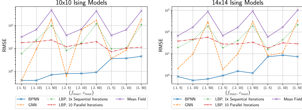
Figure 3: Each point represents the root mean squared error (RMSE, y-axis) of the specified method on a test set of 50 Ising models sampled with the parameters f_{max} and c_{max} (x-axis). The leftmost point shows results for test data drawn from the same distribution as training. BPNN significantly improves upon loopy belief propagation (LBP) for both in and out of distribution data. BPNN also significantly outperforms GNN on out of distribution data and larger models.
