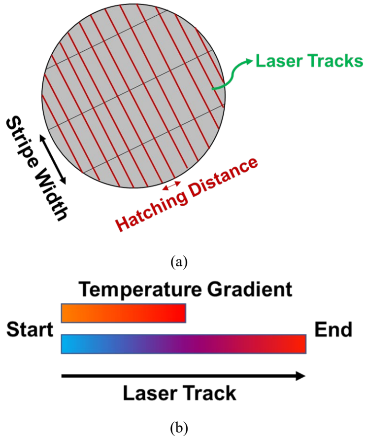
Fig. 1 (a) Schematic illustration of the stripe width, hatching distance, and laser tracks during the L-PBF process, and (b) temperature gradient in the short and long laser tracks.
