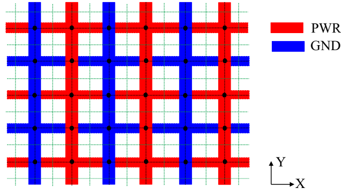
Fig. 9 P/G grid and unit cells
