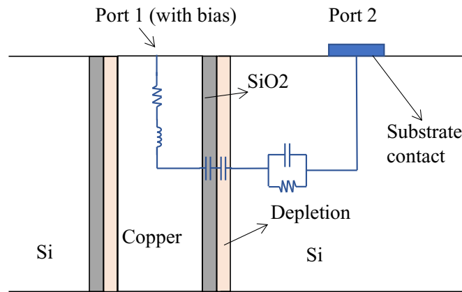
Fig.1 TSV structure and depletion region.
