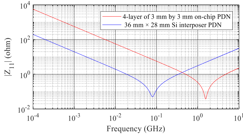
Fig. 11 Impedance of a 1-layer 6 mm \times 6 mm on-die PDN and 36 mm \times 28 mm Si interposer.
