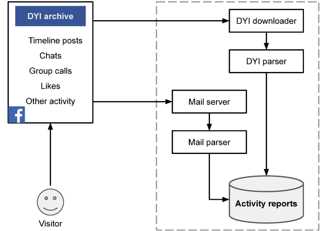
Figure 1: Monitor overview. We observe attempts to change account passwords via notification emails that arrive at our mail server, and collect records of account activity via the DYI downloader.
