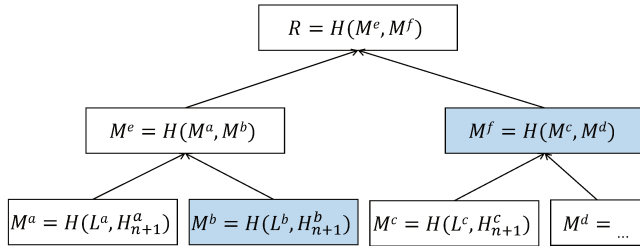
Figure 5: Merkle Hash Tree over lists a \dots d . Each leaf is a hash of the list information L^i (list name and public key) and the most recent hash of the list's hash chain H_{n+1}^i . H() is a cryptographic hash function, R is the root of the MHT, and the nodes in blue illustrate the inclusion proof path for list b .
