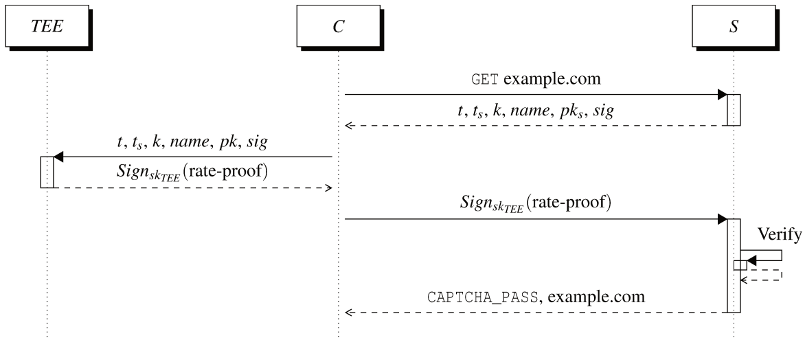
Figure 3: CACTI CAPTCHA-avoidance protocol. The client (C) requests a resource from the web server (S). In response, the server provides a timestamp for the current event ( t ), a threshold consisting of a starting time ( t_s ) and a count ( k ), and the name of the list. Optionally, the server also provides a signature ( sig ) over the request and the public key ( pk_s ) with which the signature can be verified. The client passes this information to its TEE in order to produce a rate-proof, signed by a group private key ( sk_{TEE} ), which can be verified by the server.
