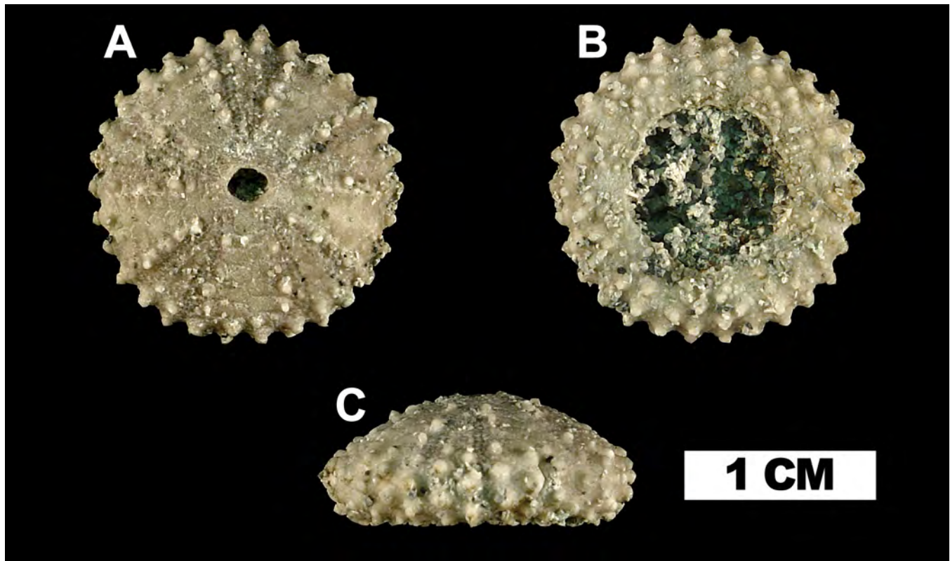
Figure 15. Arbacia improcera (UF 289215), Intracoastal Formation (FM locality LI005). A. aboral view, B. oral view, C. lateral view.
