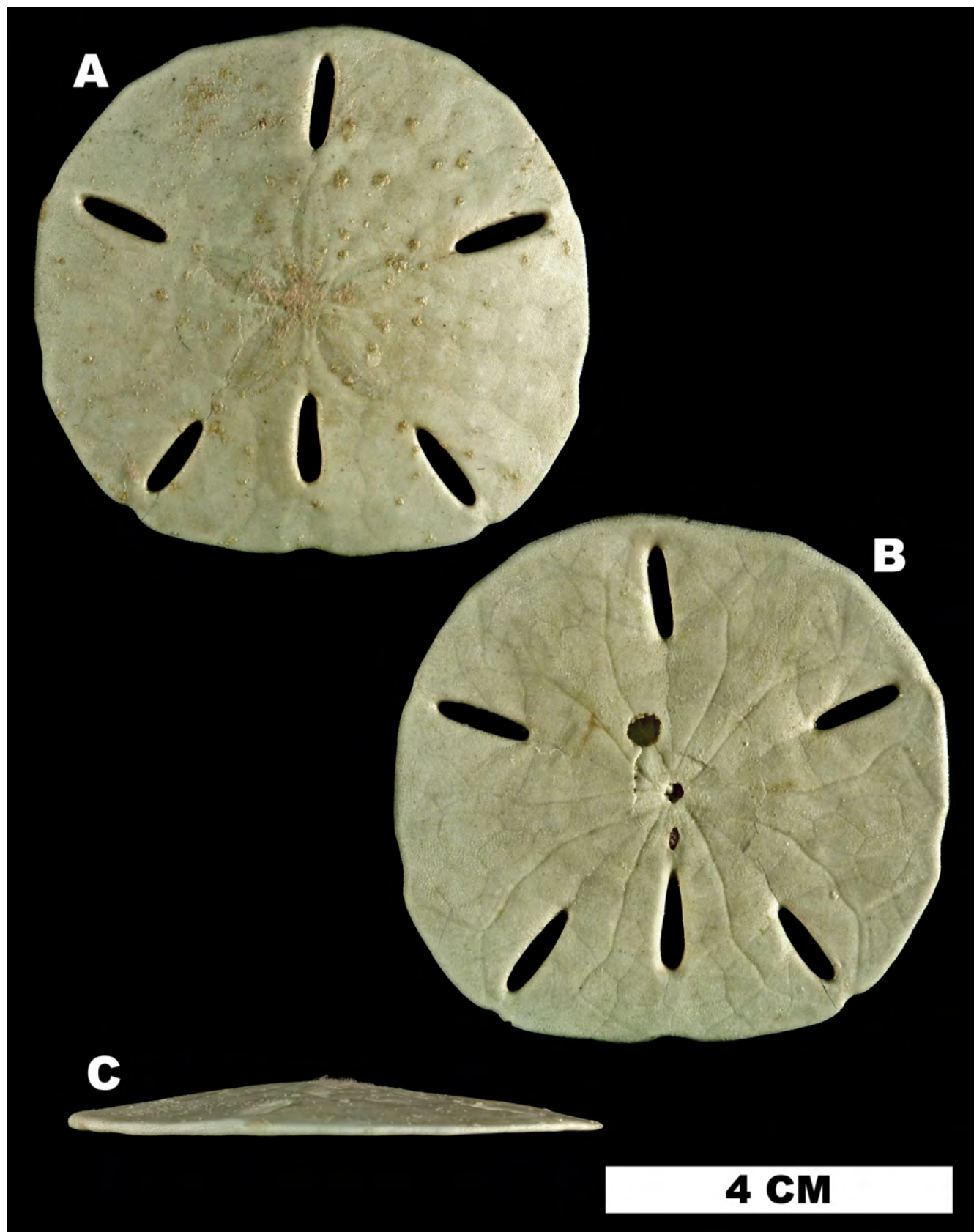
Figure 85. Leodia sexiesperforata (UF-IZ 18904), modern specimen for comparison (off Chub Cay at 2 m depth, Bahamas). A. aboral view, B. oral view, C. lateral view.
