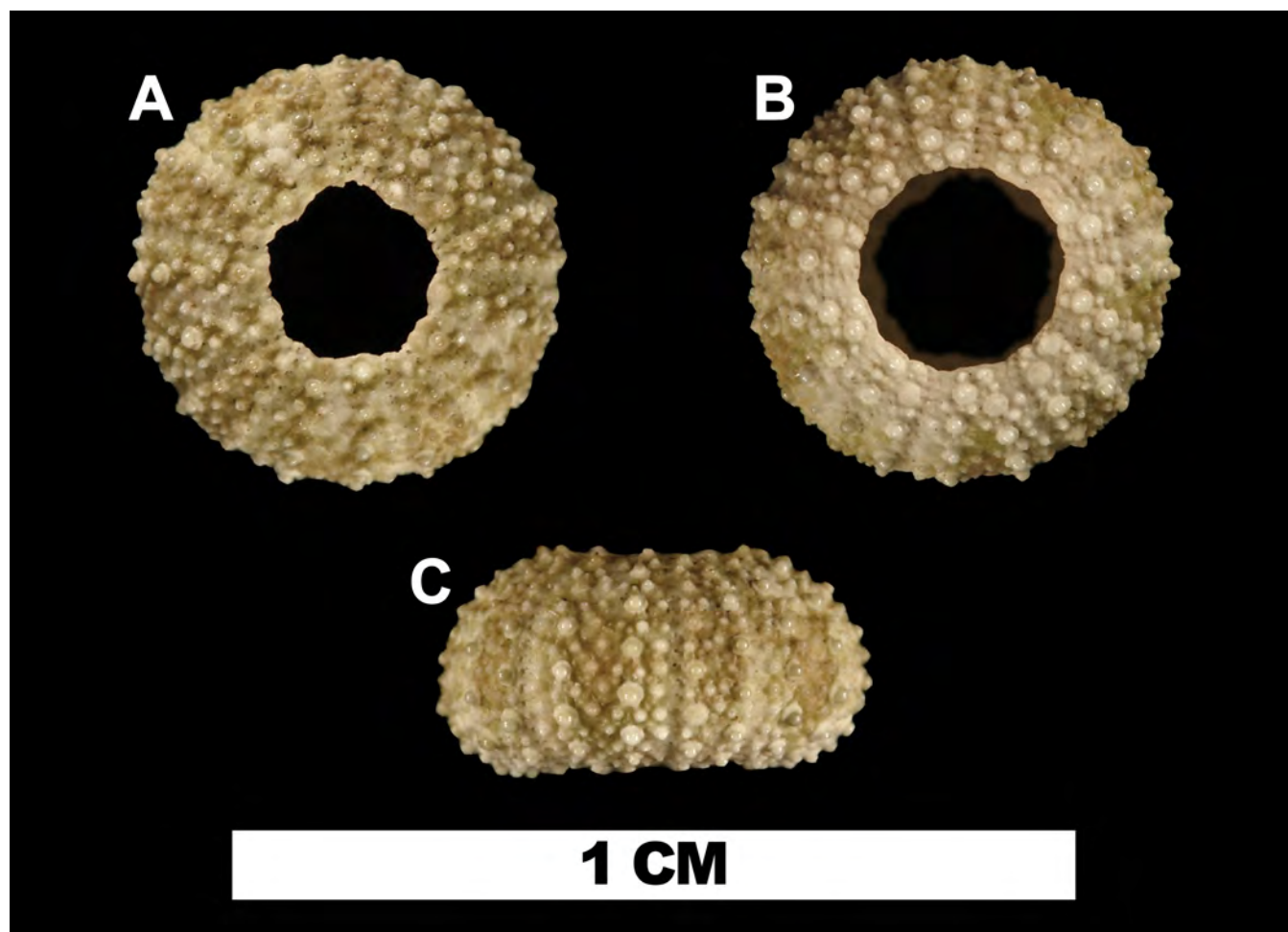
Figure 24. Genocidaris maculata (UF-IZ 18917), modern specimen for comparison from (Gulf of Mexico, 140 miles off Cape Ramano, Florida, USA). A. aboral view, B. oral view, C. lateral view.
