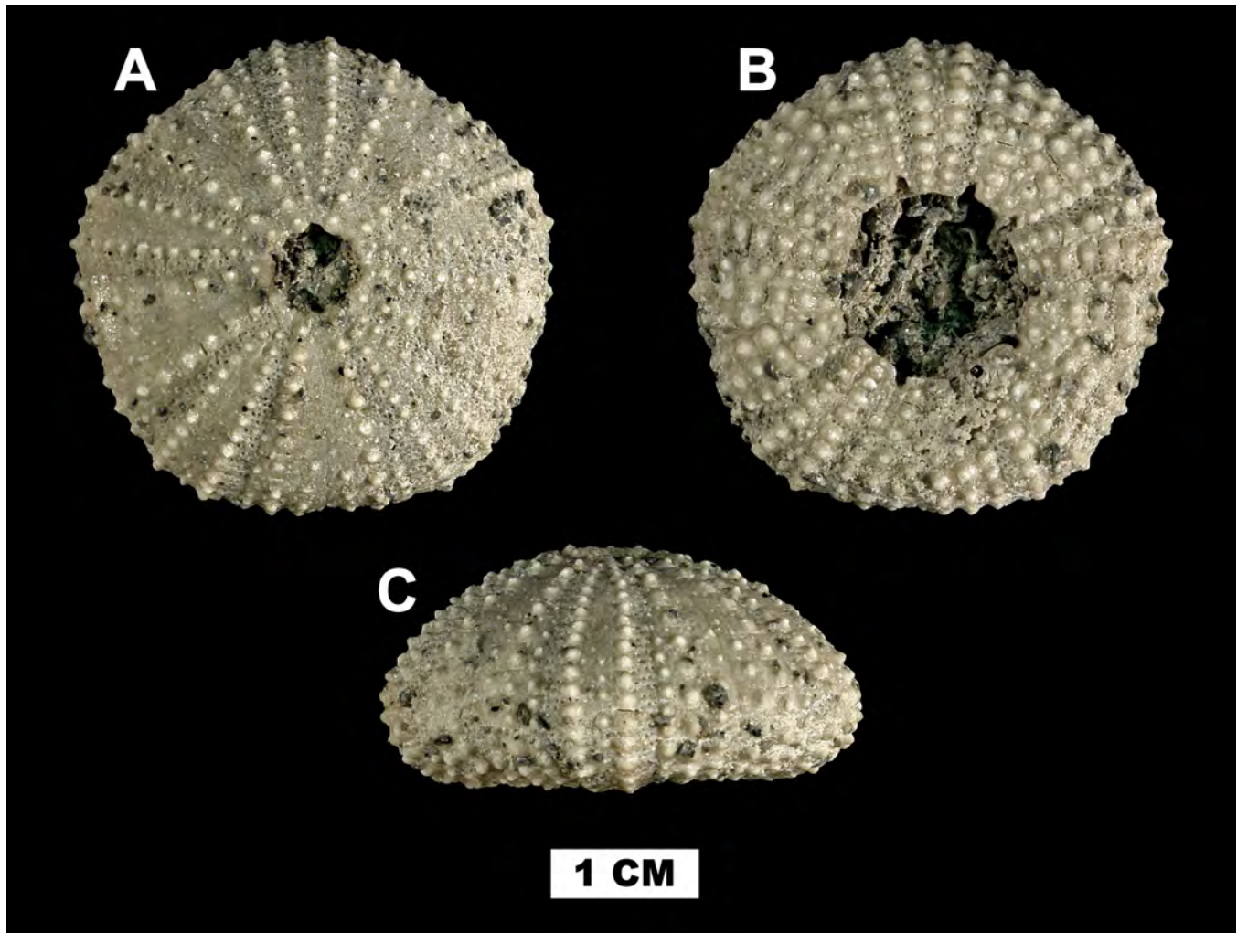
Figure 27. Lytechinus variegatus (UF 289216), Tamiami Formation (FM locality CH080). A. aboral view, B. oral view, C. lateral view.
