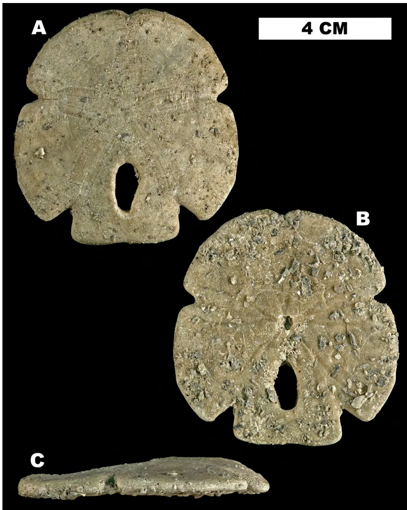
Figure 80. Encope tamiamiensis (UF 289228), Tamiami Formation (FM locality CH080). A. aboral view, B. oral view, C. lateral view.
