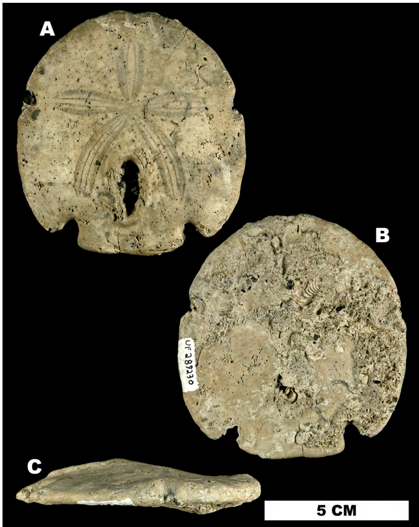
Figure 69. Encope macrophora (UF 289230), Intracoastal Formation (FM locality LI005). A. aboral view, B. oral view, C. right lateral view.
