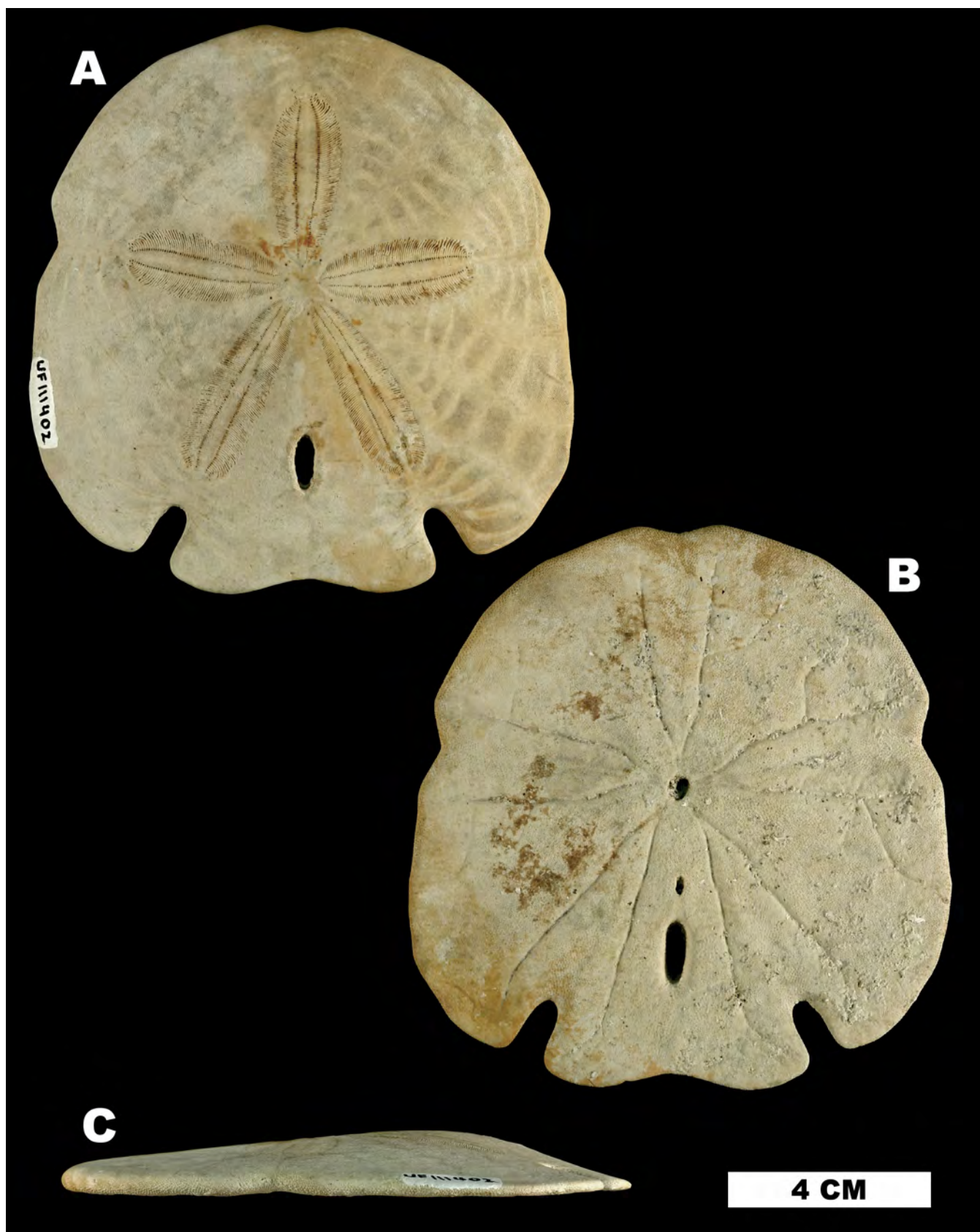
Figure 65. Encope aberrans (UF 111402), Intracoastal Formation (FM locality LI005). A. aboral view, B. oral view, C. lateral view.
