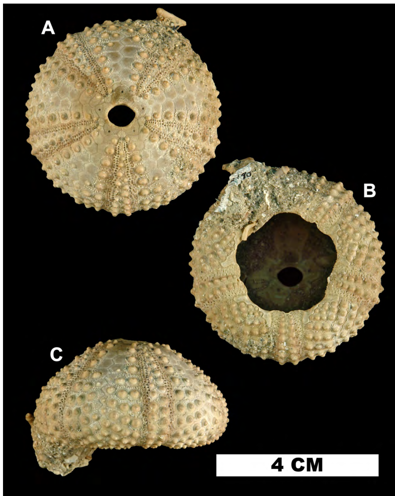
Figure 16. Arbacia punctulata (UF 112190), Anastasia Formation (FM locality SL003). A. aboral view, B. oral view, C. lateral view.
