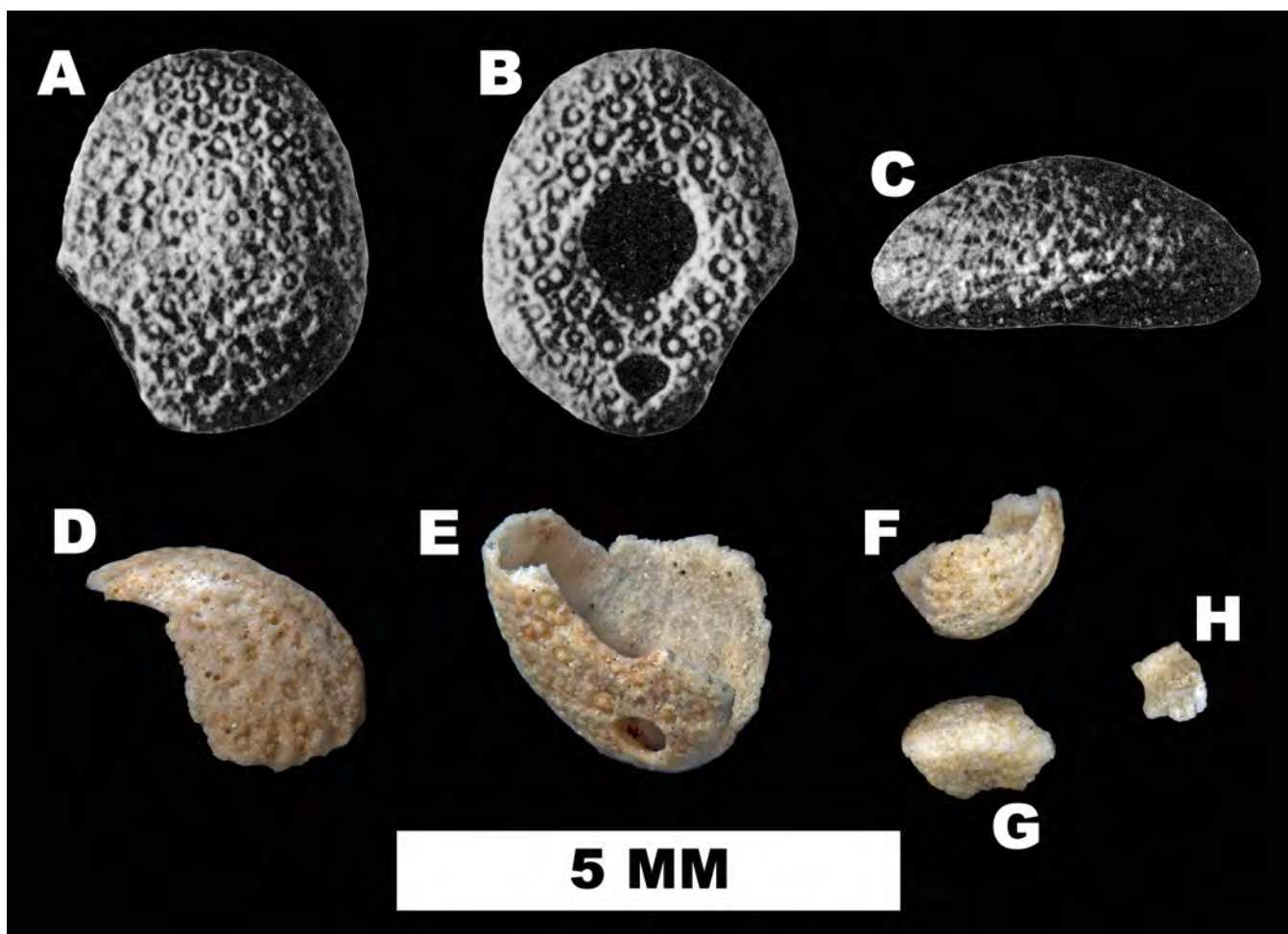
Figure 62. Echinocyamus chipolanus holotype (USNM 499003), Chipola Formation (FM locality LI003). A-C. from Cooke (1959), D-G. broken holotype.
