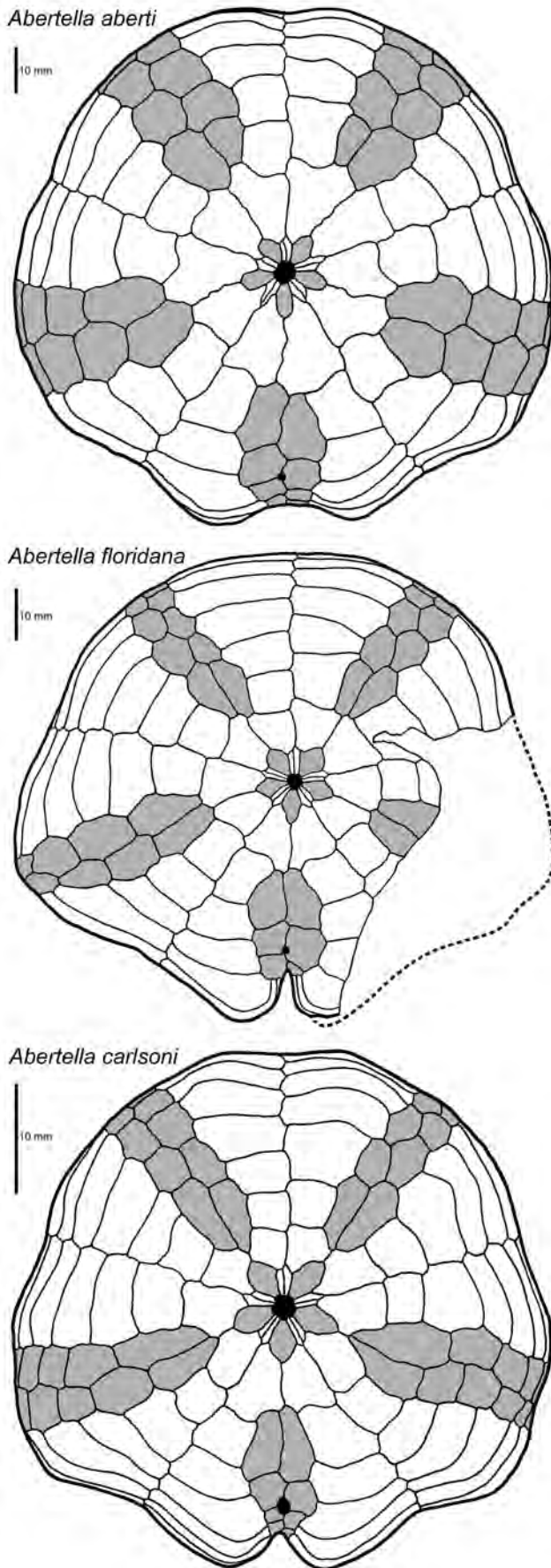
Figure 113. Comparison of oral plate architecture for Abertella aberti (CASG 91747), A. floridana (CASG 91729), and A. carlsoni (UF 284011). Anterior is towards top of page, peristome and periproct are in solid black, interambulacral plates are shaded. Outline of left side of test reconstructed with dotted line for A. floridana .
