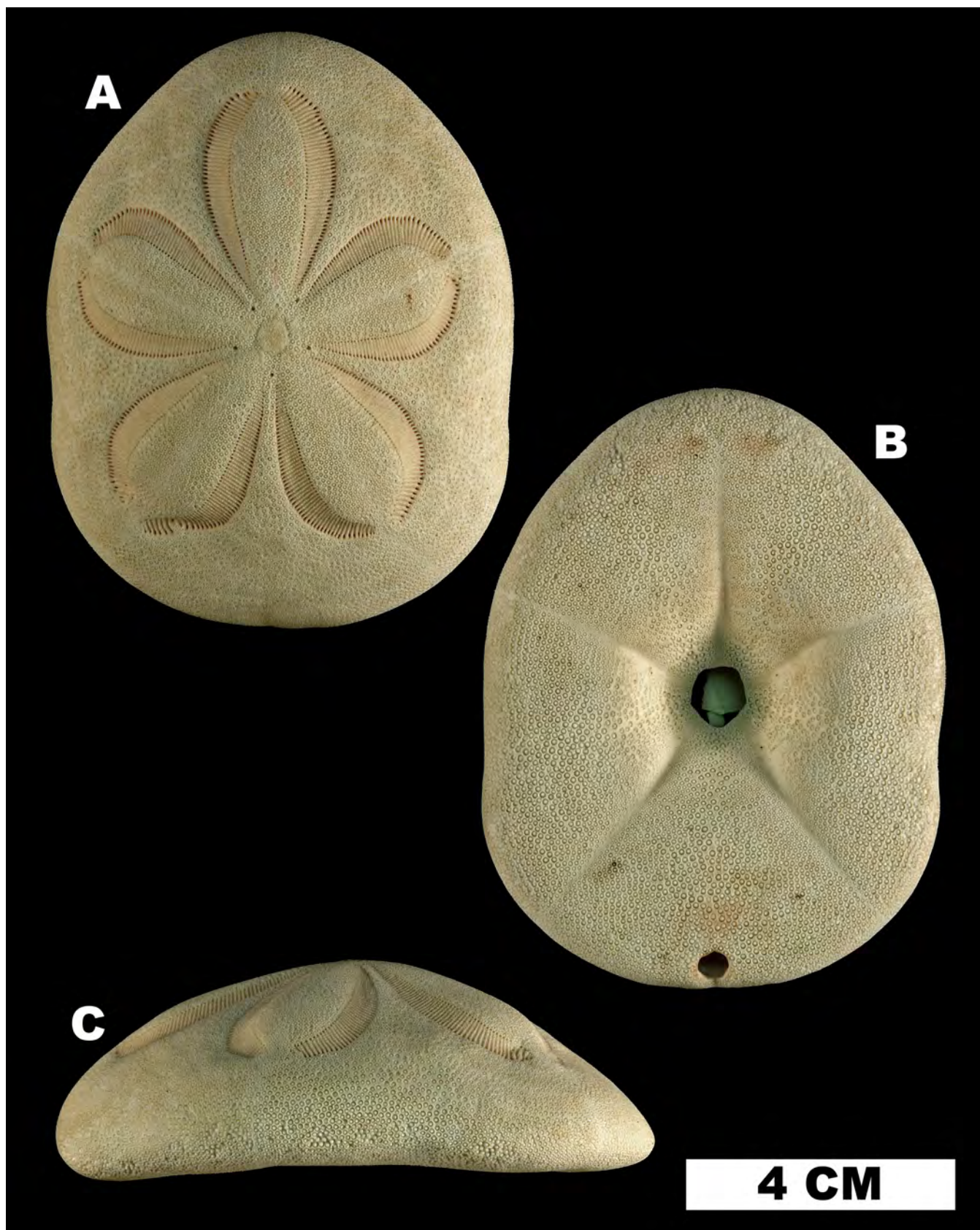
Figure 50. Clypeaster rosaceus (UF-IZ 18900), modern specimen (off Marathon Key at 2 m depth, Monroe County, Florida, USA). A. aboral view, B. oral view, C. lateral view.
