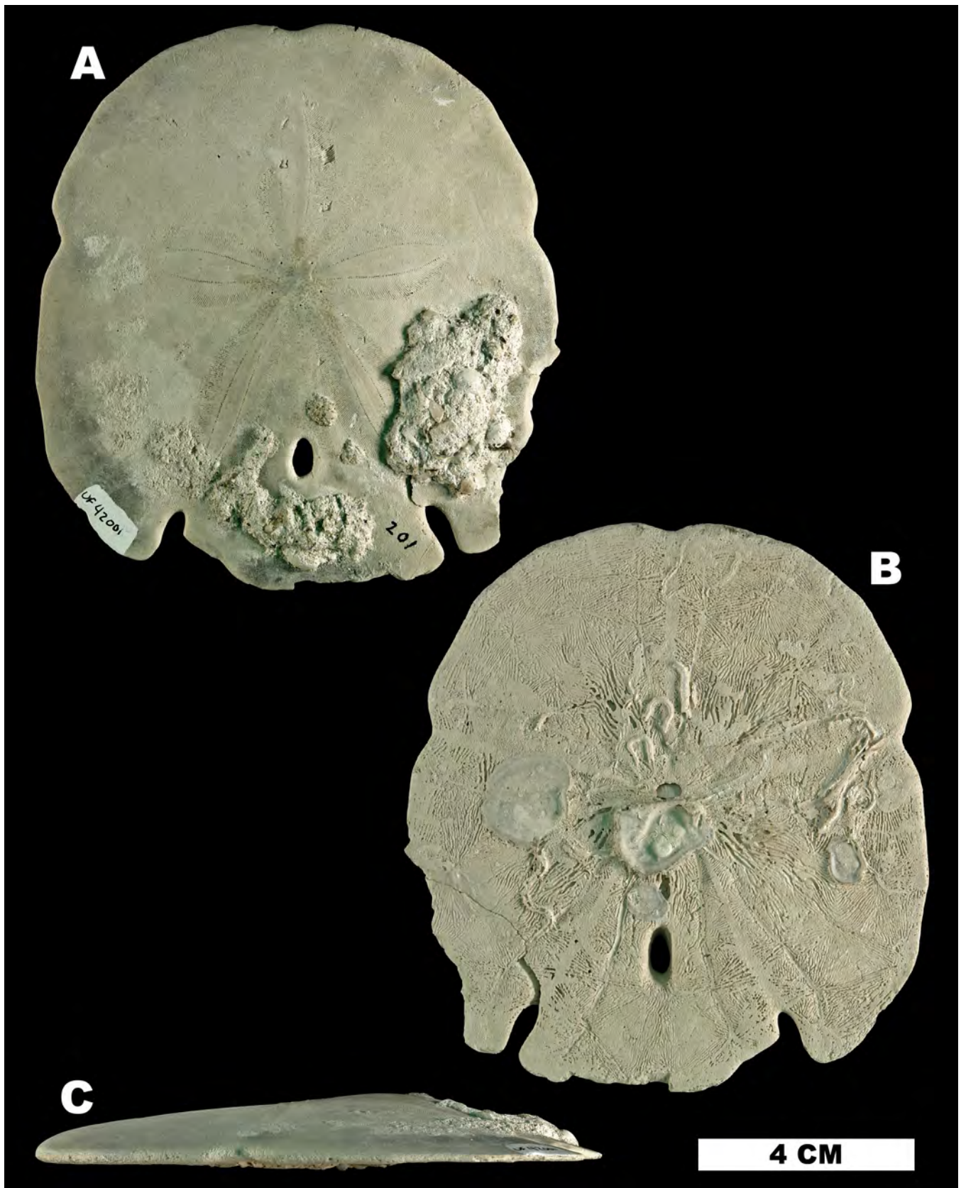
Figure 67. Encope aberrans (UF 42001), Bermont Formation (FM locality PB001). A. aboral view, B. oral view, C. lateral view.
