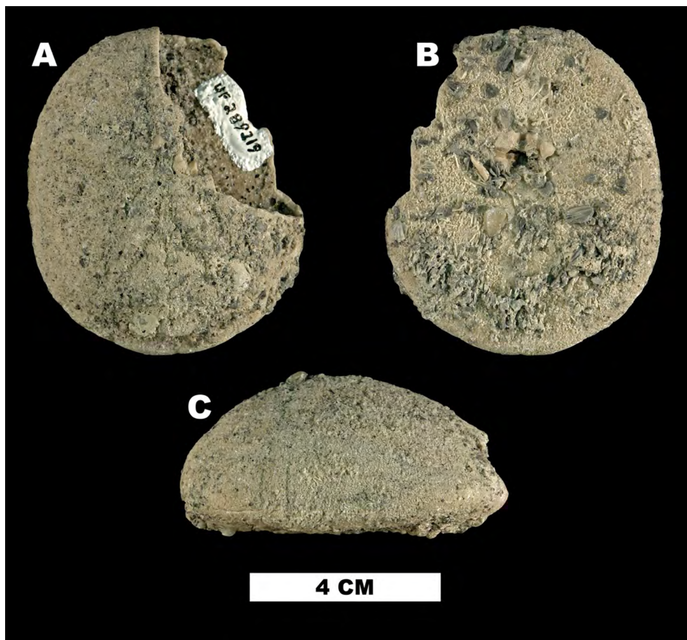
Figure 40. Rhyncholampas evergladensis with spines (UF 289219), Tamiami Formation (FM locality CH080). A. aboral view, B. oral view, C. lateral view.
