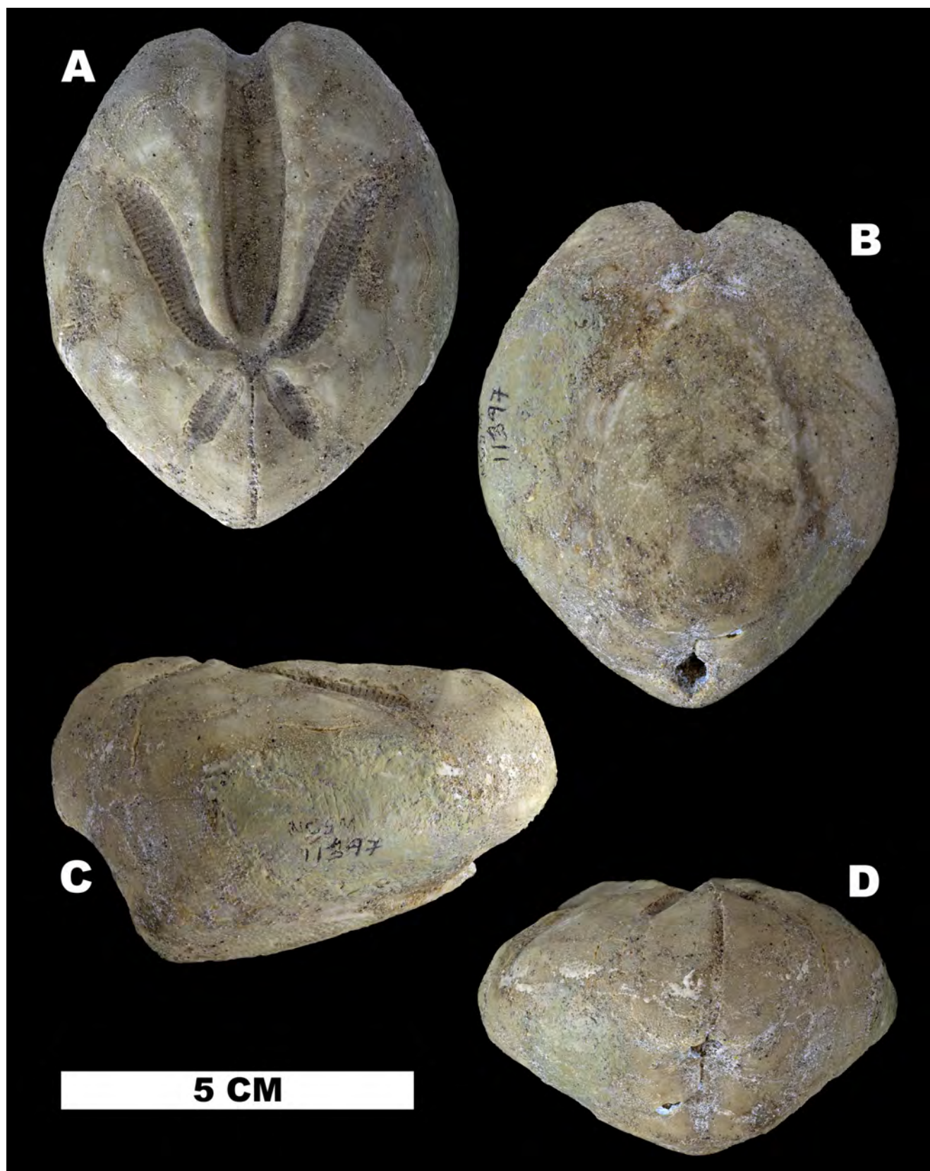
Figure 142. Schizaster kieri holotype (NCSM 11397), Intracoastal Formation (FM locality LI005). A. aboral view, B. oral view, C. right lateral view, D. posterior view.
