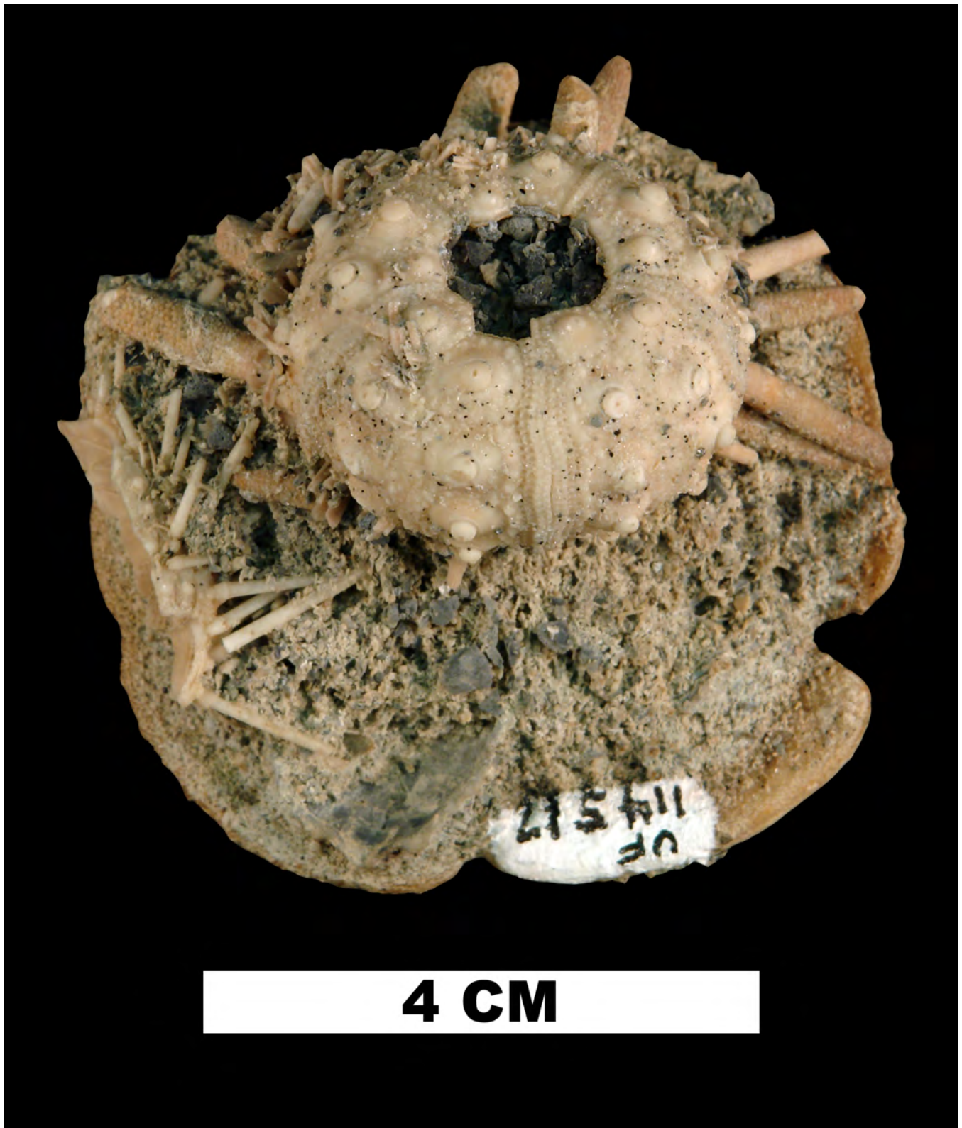
Figure 6. Eucidaris tribuloides (UF 114517) with attached spines (Aboral view), Encope tamiamiensis (underneath), and attached to left side Lytechinus variegatus , Tamiami Formation (FM locality CH046).
