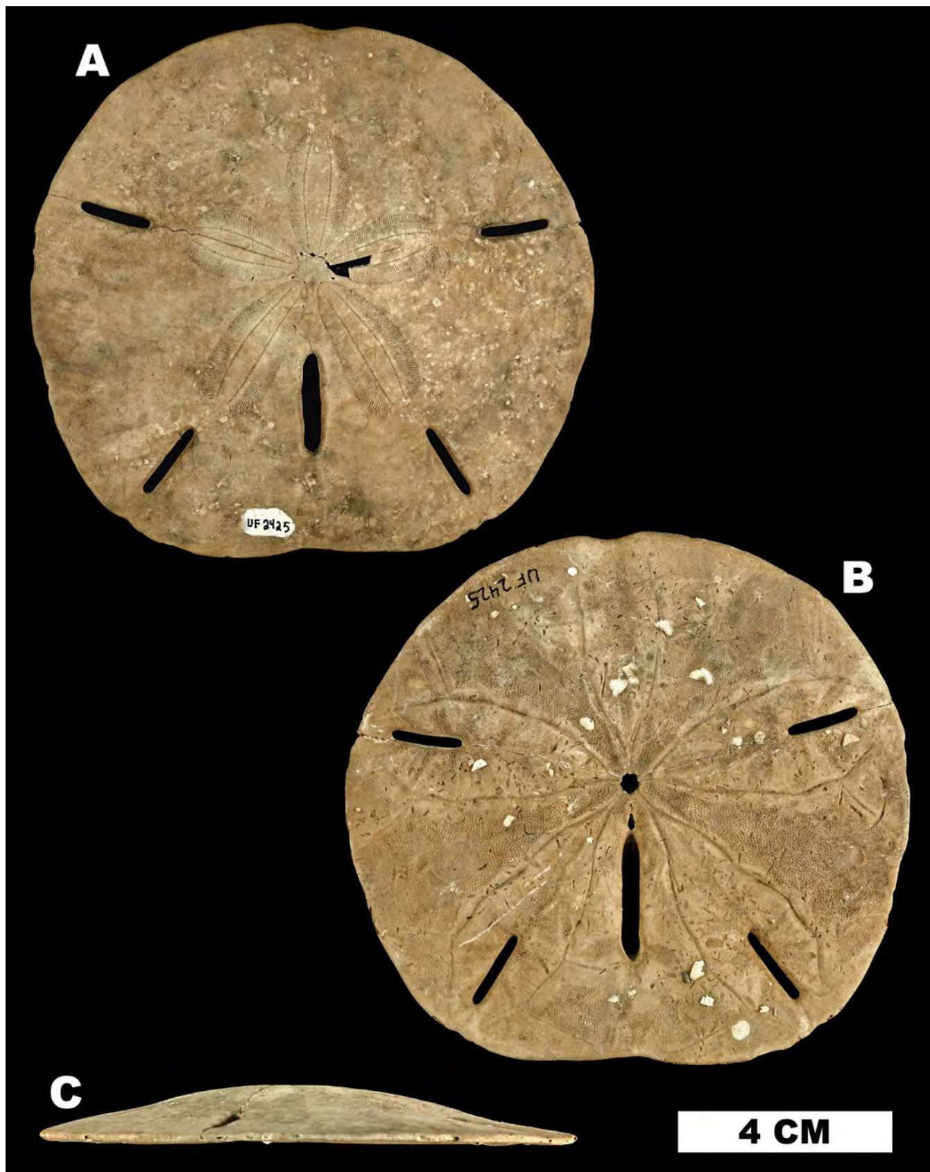
Figure 92. Mellita isometra (UF 2425), undifferentiated Pleistocene strata (FM locality MA004). A. aboral view, B. oral view, C. lateral view.
