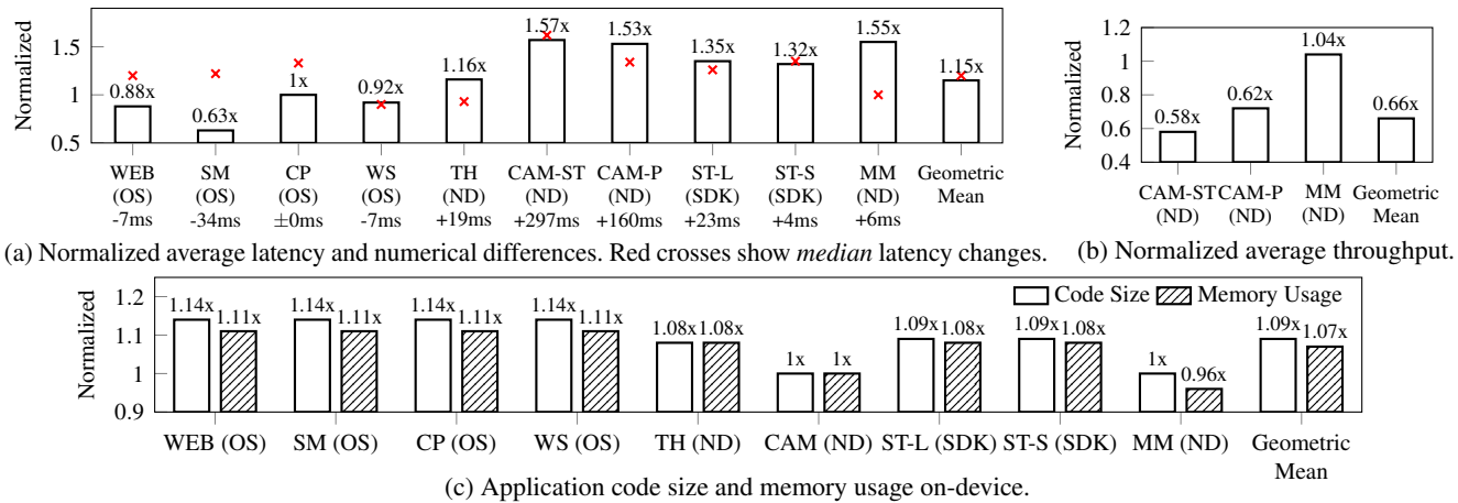
Figure 8: Performance overhead for all prototype apps. Data are normalized to results from the original apps. CAM has two modes: S teaming videos and taking P ictures. We denote integration approaches in parentheses: OS Replacement, Native Driver, and Framework SDK Replacement. Based on geometric means, Figure (a) shows a 15% latency increase and Figure (b) shows a 34% throughput reduction. Figure (c) shows the Capture-enabled firmware incur around 10% more on-device resource utilization.
