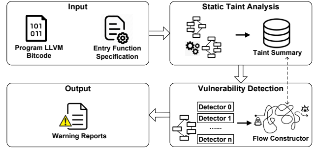
Figure 2: System Architecture of SUTURE
