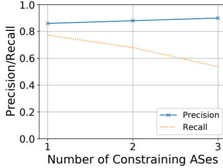
Fig. 7. Impact of the number of constraining ASes, i.e. , |\mathcal{B}| , on recall and precision. More constraining ASes limit where chosen paths are received by a target AS T , improving precision, but fewer AS paths are long enough to support many constraining ASes, reducing recall.
