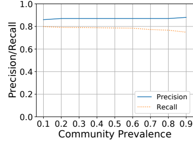
Fig. 5. Precision and recall as a function of K_{\text{prev}} . Location communities appear on most routes in \mathcal{R}(V, \mathcal{A}, T, \mathcal{B}) , so increasing K_{\text{prev}} up to 0.9 has small impact on precision and recall.
