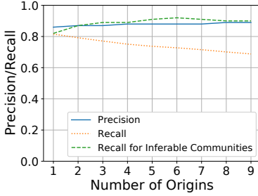
Fig. 4. Precision and recall as a function of K_{\text{origins}} . High precision for K_{\text{origins}} = 1 indicates that origins rarely tag all their announcements with traffic engineering communities of other ASes.
