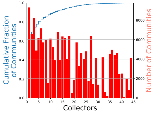
Fig. 3. Number of inferred communities and recall as a function of the number of collectors.
