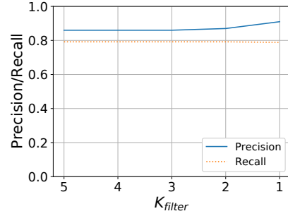
(b) Precision and recall as a function of K_{\text{filter}}
