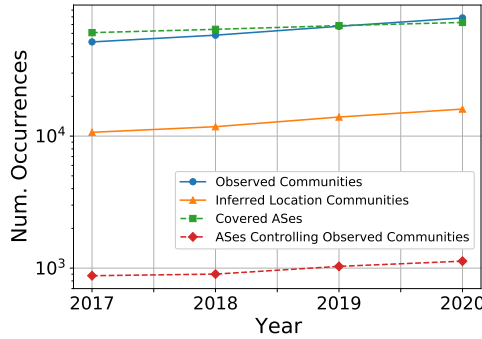
Fig. 8. BGP community use in the Internet, quantified as the number of distinct BGP communities observed, number of inferred location communities, and the number of ASes controlling BGP communities.
