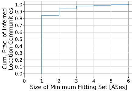
(a) Distribution of minimum hitting set sizes
