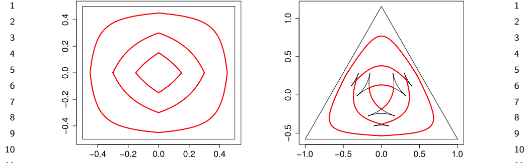
FIG 6. Curves of barycenters of hyperplanes that cut off volume \delta \in \{0.05, 0.20, 0.35\} from convex bodies (thin black lines), and the boundaries of convex floating bodies for the same values of \delta (thick red lines), for the uniform distribution on a square (left panel) and a triangle (right panel). For the square, all (Dupin's) floating bodies exist, and coincide with the convex floating bodies. For the triangle, the boundaries of all convex floating bodies are proper sub-curves of the corresponding black curves (the difference is not visible in the plot for \delta = 0.05 ). The (Dupin's) floating bodies do not exist.
