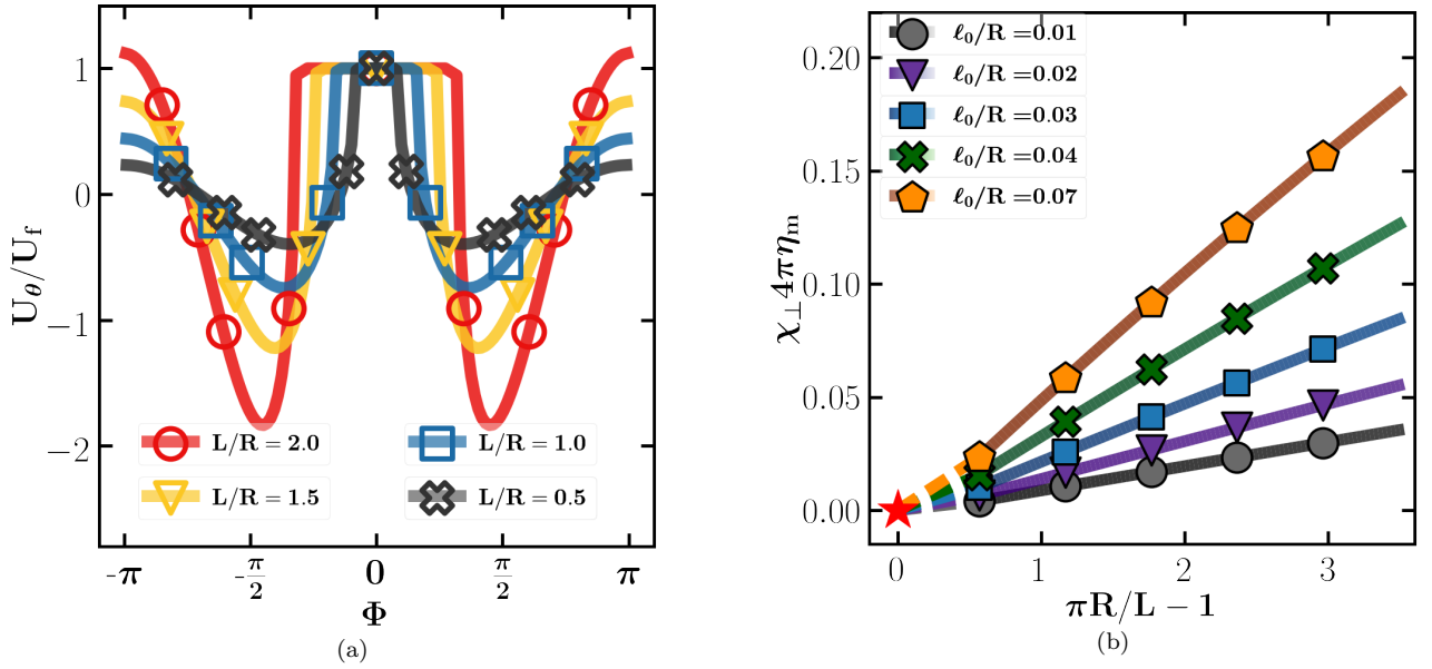
FIG. 4. (a) The polar velocity distributed in the azimuthal direction along the equator, normalized by the filament velocity for the choice of \ell_0/R = 1 . The different colors/symbols represent different ratios of L/R . (b): The mobility of filament in perpendicular direction as a function of gap distance, \epsilon = \pi R/L - 1 for different values of \ell_0/R .
