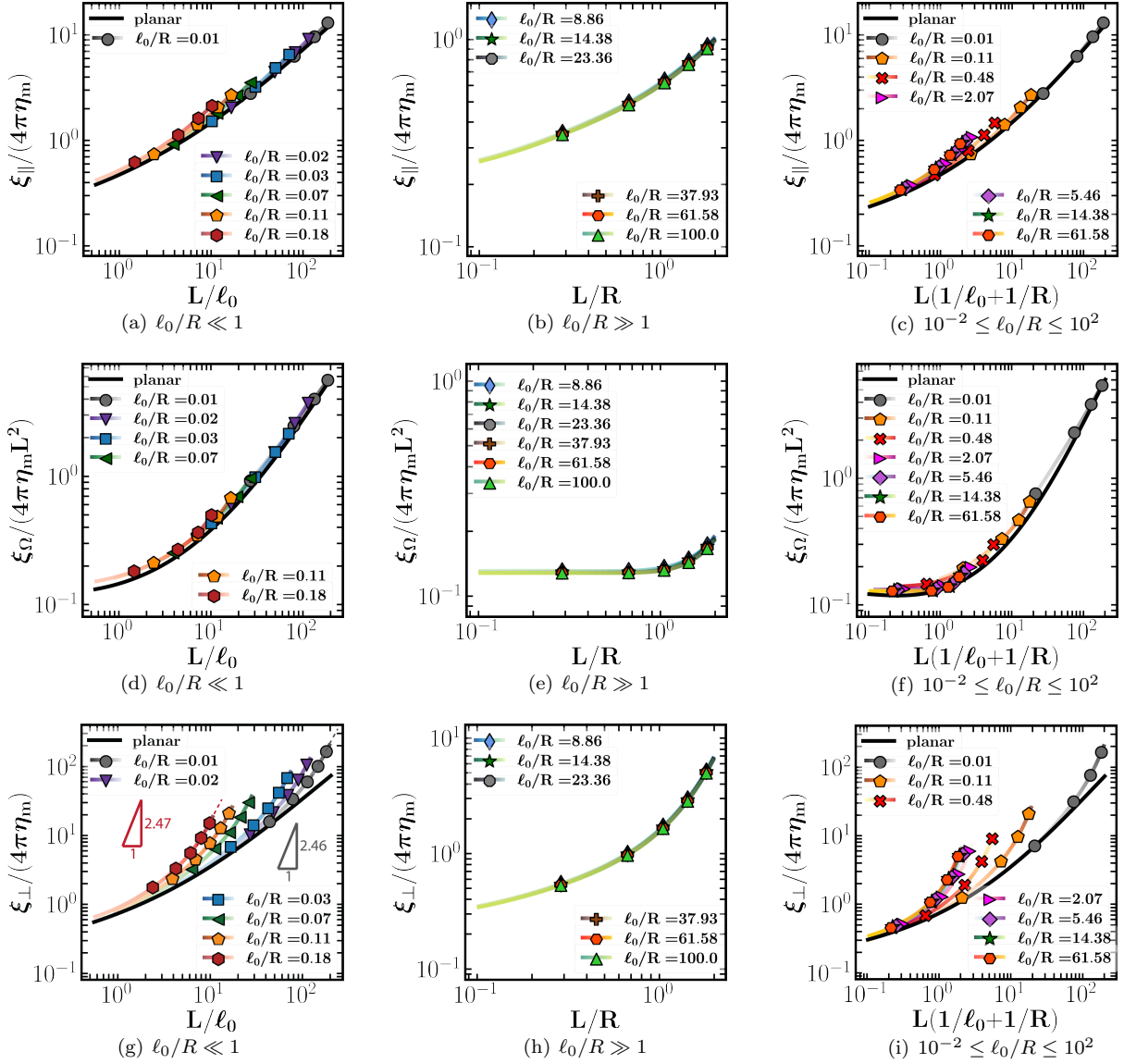
FIG. 2. The parallel, perpendicular and rotational resistance as a function of L/\ell_0 and L/R in different limits of \ell_0/R . The upper, middle and lower rows represent resistance in the parallel, rotational and perpendicular direction, respectively. The left column and middle column correspond to \ell_0 \ll R and \ell_0 \gg R , respectively. The right column includes all data in the range 10^{-2} \leq \ell_0/R \leq 10^2 . The solid black lines in (a), (d) and (g) represent the associated resistance values in planar membranes [22]. The variations of L/R for each choice of \ell_0/R is visualized by changing the color from light (left-end of each plot) to dark (right-end of each plot) with increasing L/R .
