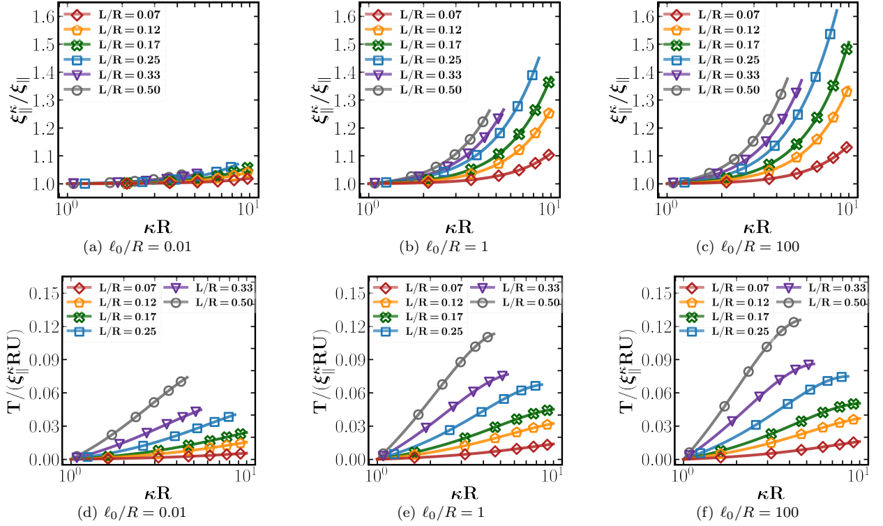
FIG. 6. Top row (a-c): The resistance along the parallel direction vs the filament's dimensionless curvature ( \kappa R ) for 0.07 \leq L/R \leq 0.50 at (a) \ell_0/R = 0.01 , (b) \ell_0/R = 1 and (c) \ell_0/R = 100 . When \ell_0/R \ll 1 the parallel resistance remains nearly constant with curvature and equal to the results at the equator. When \ell_0/R \geq 1 , the resistance monotonically increases with curvature, and the rate of this increase is amplified with increasing L/R . Bottom row (d-f): the net torque induced on the filament by its motion in the parallel direction as a function of the filament's dimensionless curvature for the range 0.07 \leq L/R \leq 0.50 at (d) \ell_0/R = 0.01 , (e) \ell_0/R = 1 and (f) \ell_0/R = 100 . The torque magnitude is non-dimensionalized by the external force moment on the membrane: \xi_{\parallel}^R RU . Regardless of the choice of \ell_0/R , the torque monotonically increases with \kappa R ; this effect is amplified with increasing L/R . The results appear to be a weak function of \ell_0/R and the torque remains < 15\% of the external force moment.
