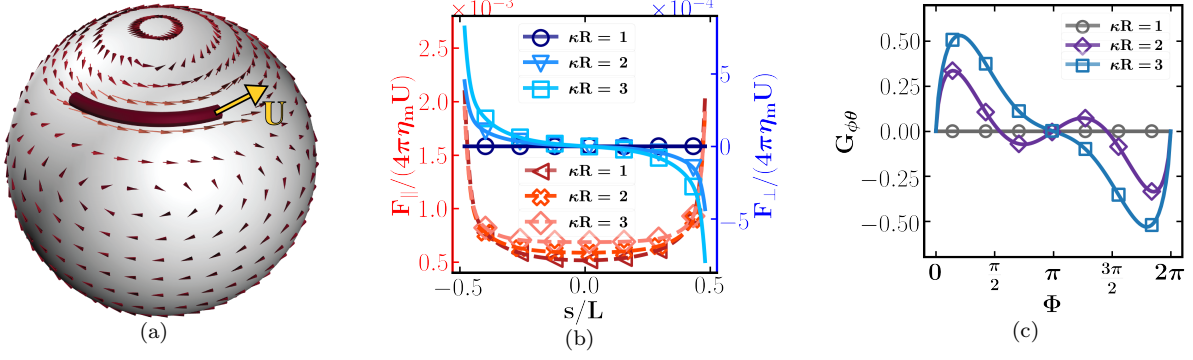
FIG. 5. (a) The flow field induced by the parallel motion of a filament placed at h = R/\sqrt{2} away from the equator ( \kappa = \sqrt{2}R^{-1} ), when \ell_0/R = 1 and L/R = 1 . (b) The distribution of force per unit length along the filament in parallel and perpendicular directions ( \mathbf{f}_{\parallel,\perp} ) at different latitudes (curvatures), when \ell_0/R = 1 and L/R = 1 . (c) Variations of G_{\phi\theta} vs \phi , at different latitudes/curvatures ( \theta_0 ), when the source point is located at (\theta_0, \phi_0 = 0) and the target is at (\theta_0, \phi) . The results are presented for \ell_0/R = 1 ; see Appendix A for the full expression of the Green's function.
